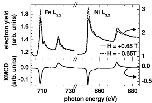
FIG. 1. (a) Fe and Ni L_{3,2} spectra of a 20 Å Ni/500 Å FeF 2 bilayer measured at T=55 K. Spectra obtained for parallel and antiparallel orientation of external field and photon helicity are indicated by a dotted and a solid line, respectively. (b) XMCD spectrum of the same sample, that is, the difference of the spectra shown in (a).
