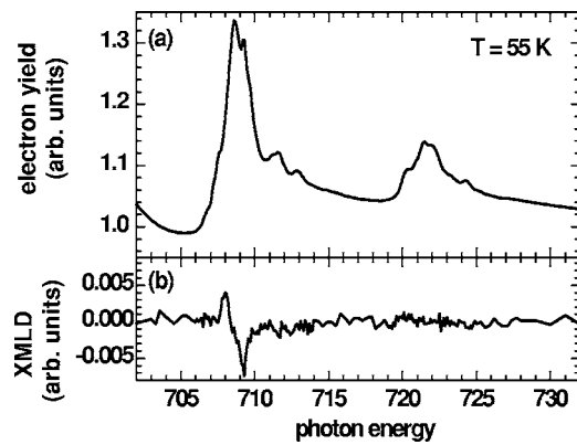
FIG. 3. (a) Fe L_{3,2} spectrum measured in normal incidence with linearly polarized x-rays at T=55 K. The average of spectra obtained with the polarization axis parallel and perpendicular to the \text{FeF}_2(001) direction is shown. (b) XMLD spectrum; that is, the difference of the spectra observed in normal incidence by switching a magnetic field of 0.65 T in the sample plane between parallel and perpendicular to the polarization axis of the linearly polarized x rays.
