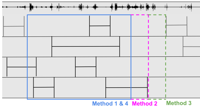
Figure 2: Visualization of audio segmented into utterances and partitioned by speaker. Different sampling methods treat sampling boundaries that fall within utterances differently. Sampling methods 1 & 4 retain the generated sampling boundary (in blue), while methods 2 and 3 extend the boundary (in pink and green, respectively).
