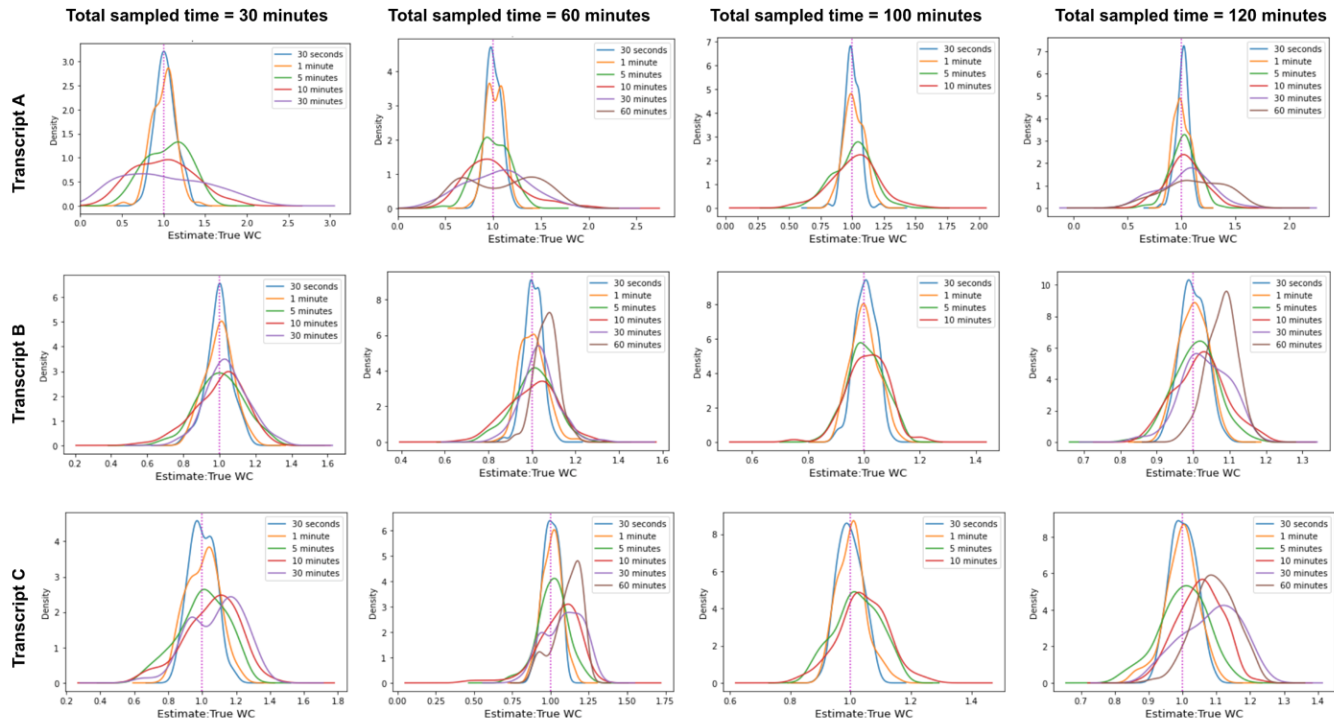
Figure 4: Kernel distribution estimation plots of the proportion of the estimated daylong word count to the true daylong word count for select total sampled times (30 minutes, 60 minutes, 100 minutes, 120 minutes) across different sampling interval sizes (30 seconds up to 60 minutes; see Legend) over 100 simulations. A dotted line at x = 1.0 is included for interpretability. The first row presents these results for Transcript A, the second for Transcript B, and the third for Transcript C.
