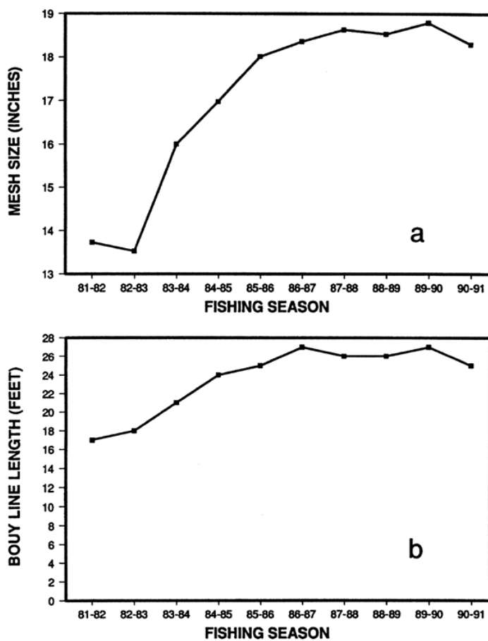
FIGURE 6. Average mesh size in inches (a) and buoy-line length in feet (b) used by California drift gill net vessels during the 1981-82 through 1990-91 fishing seasons.
