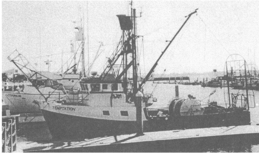
FIGURE 4. California drift gill net vessel with swordfish plank and pulpit at the bow, crow's nest atop the mast, net reel amidships, and net guard raised above the stern.
