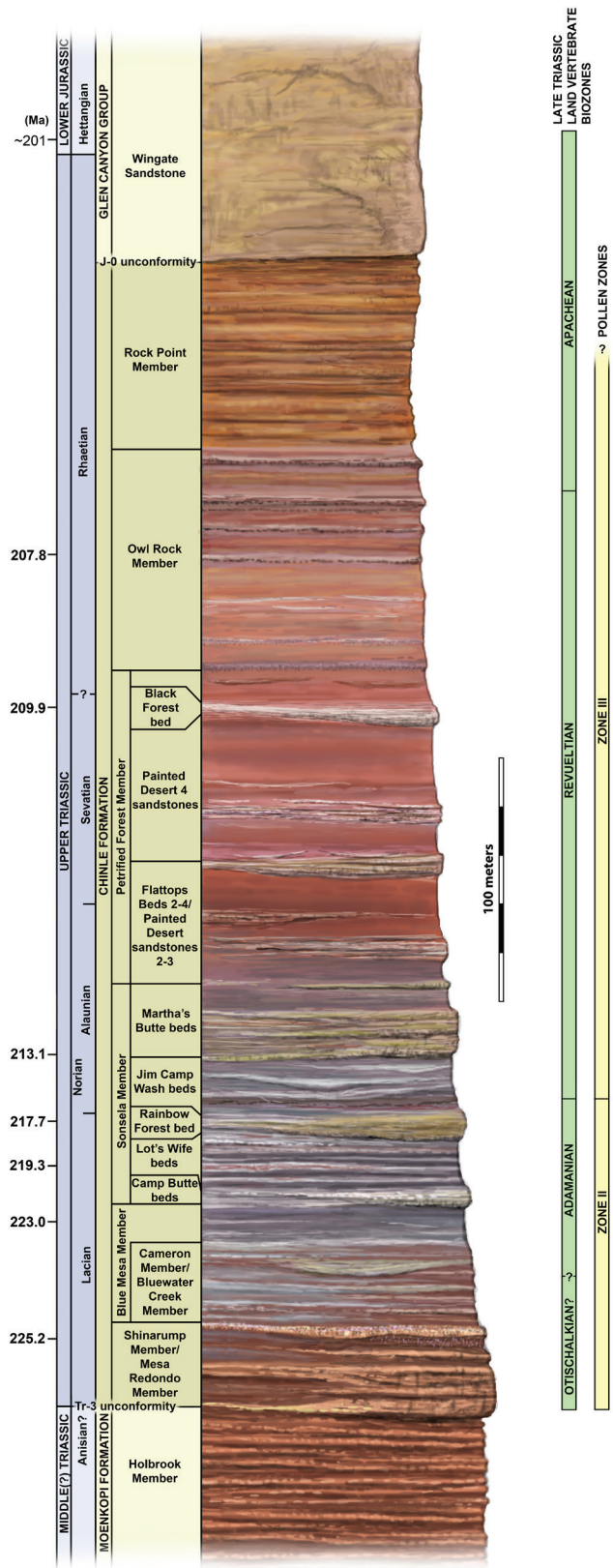
FIGURE 1. General stratigraphy of the Chinle Formation in northeastern Arizona based on geological mapping, stratigraphic correlations, and U-Pb geochronology. JEFFREY MARTZ
