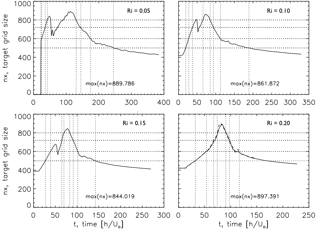
Figure 1: Time-evolving resolution requirements per wavelength \lambda for Ri=0.05 , Re=2500 (upper left), Ri=0.10 , Re=2800 (upper right), Ri=0.15 , Re=2900 (lower left), and Ri=0.20 , Re=4000 (lower right).
