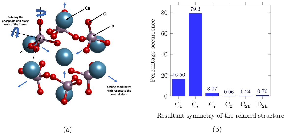
Figure 1: (a) The scheme used for creating over 10,000 structures by rotating the phosphate units and scaling all the coordinates with respect to central atom. The blue, purple, and red spheres represent Ca, P, and O atoms respectively. (b) Percentage occurrence of each point group symmetry after ab initio structural relaxation of over 10,000 initial structures (DFT with B3LYP hybrid functional and 6-311G(d,p) basis set).
