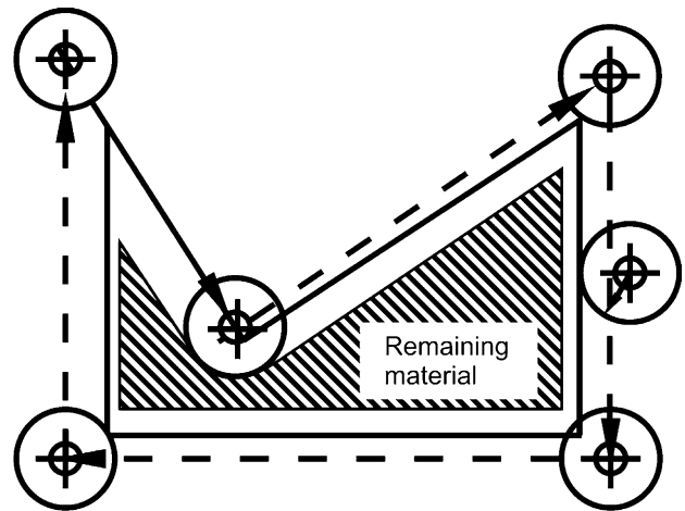
Fig. 33. Window framing [57].
