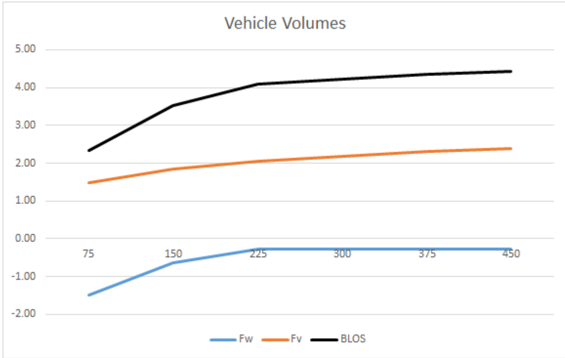
Figure 20: Sensitivity of link BLOS to variations in traffic volume.
