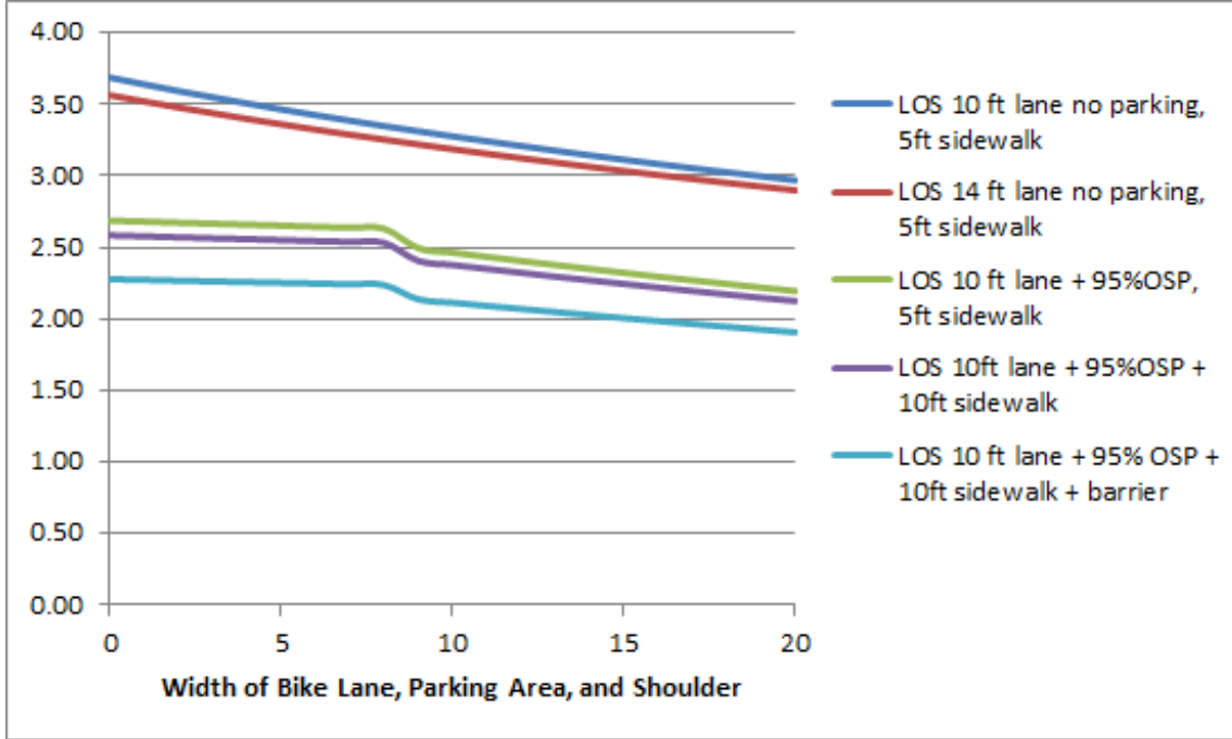
Figure 13: Effect of various components of F_w on Link PLOS.
