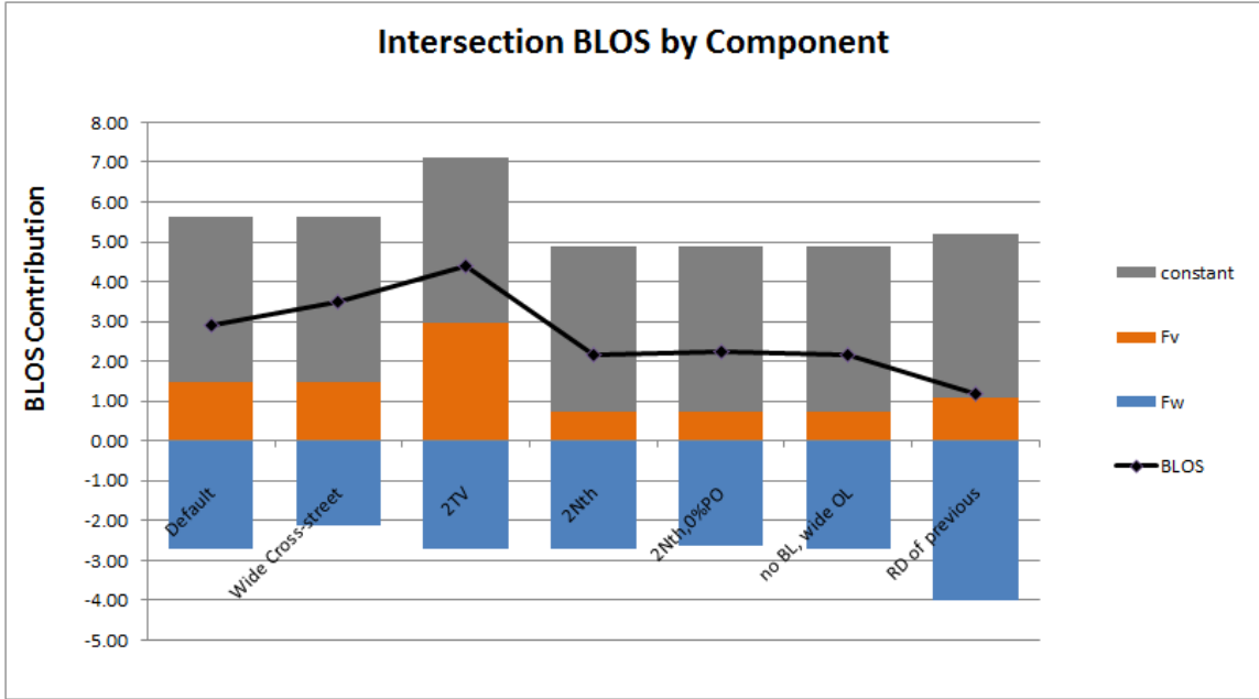
Figure 16: Contributions of F_w , F_v and the constant to intersection BLOS for a variety of cases.
