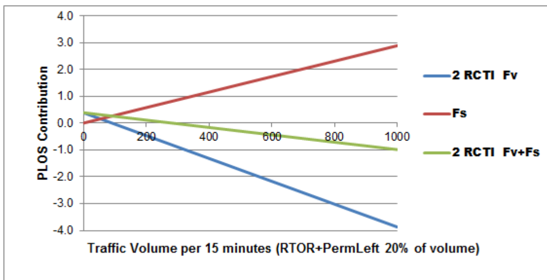
Figure 6: Intersection PLOS as a function of vehicle volumes.
