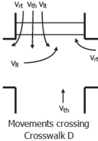
Figure 3: Vehicular movements in potential conflict with the subject crosswalk. Source: 2010 Highway Capacity Manual, page 18-70
