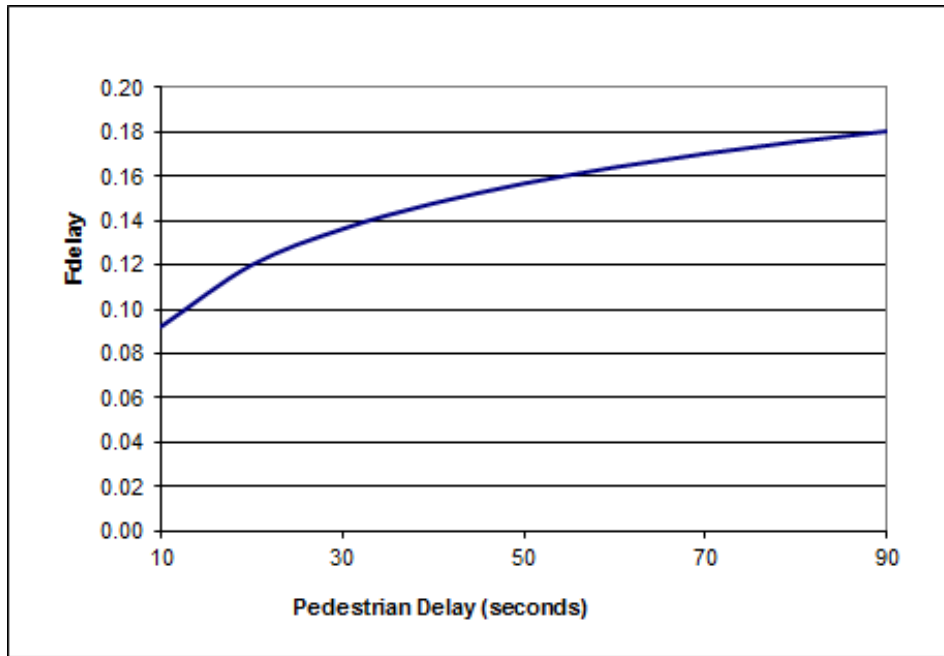
Figure 8: Intersection PLOS as a function of pedestrian delay.
