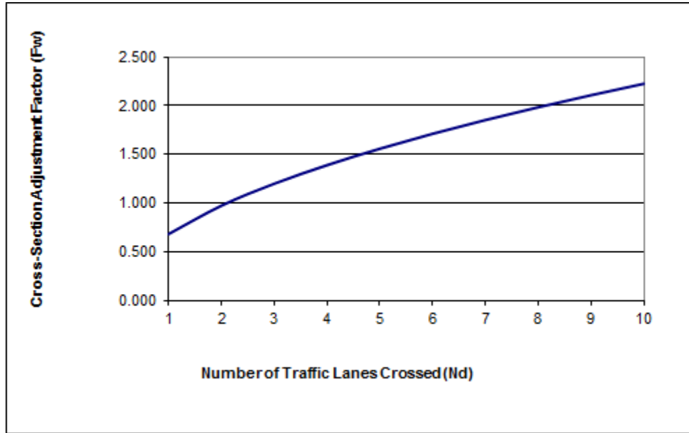
Figure 5: Intersection PLOS as a function of number of traffic lanes crossed.
