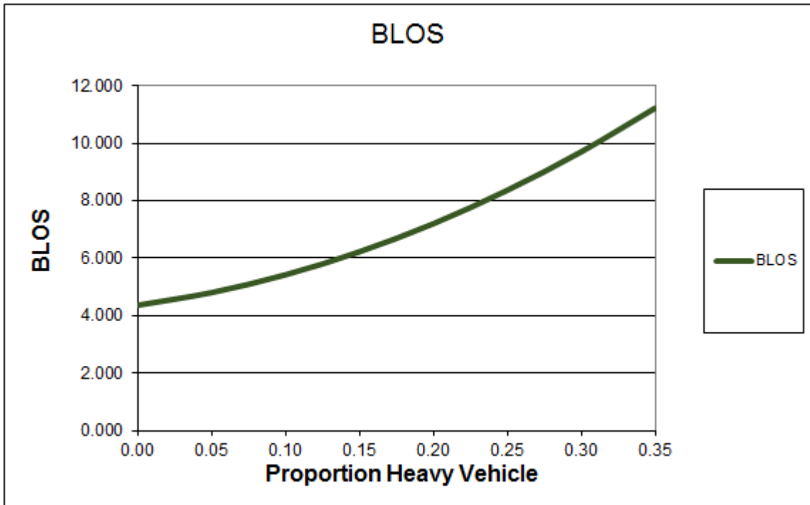
Figure 23: Sensitivity of Link BLOS to variations in the percentage of heavy vehicles.
