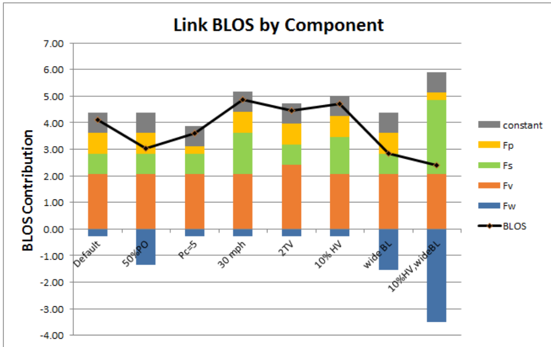
Figure 19: Contributions of F_w , F_v , F_s , F_p and the constant to link BLOS for a variety of cases.
