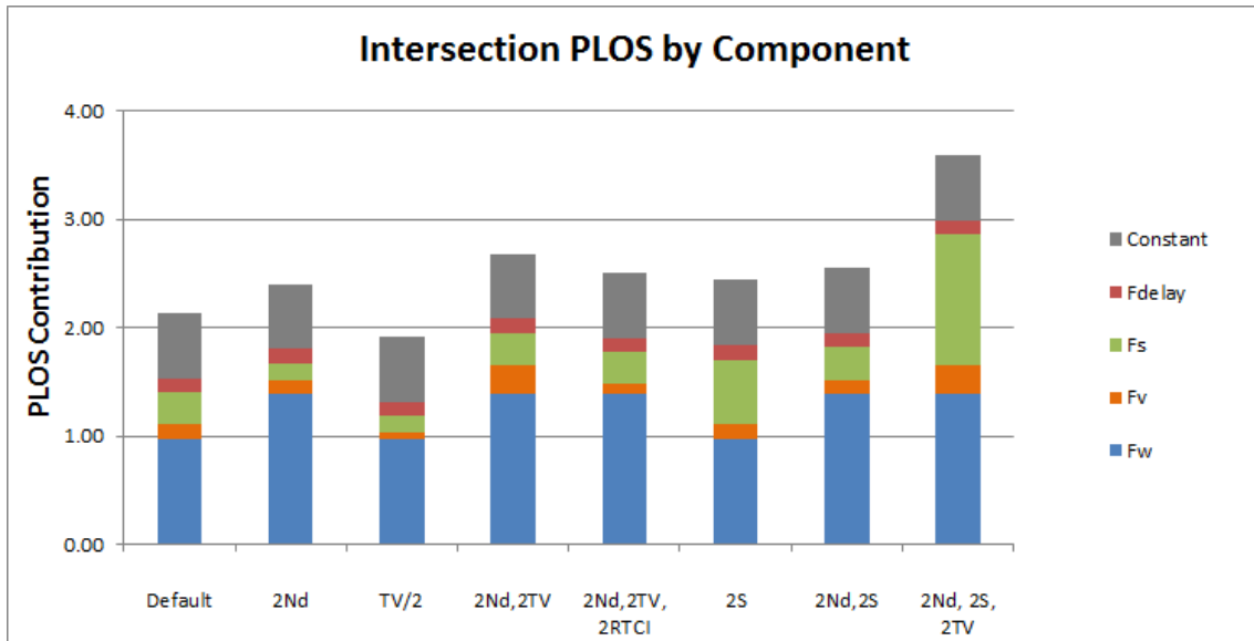
Figure 4: Contribution of component factors to intersection PLOS in a variety of cases.
