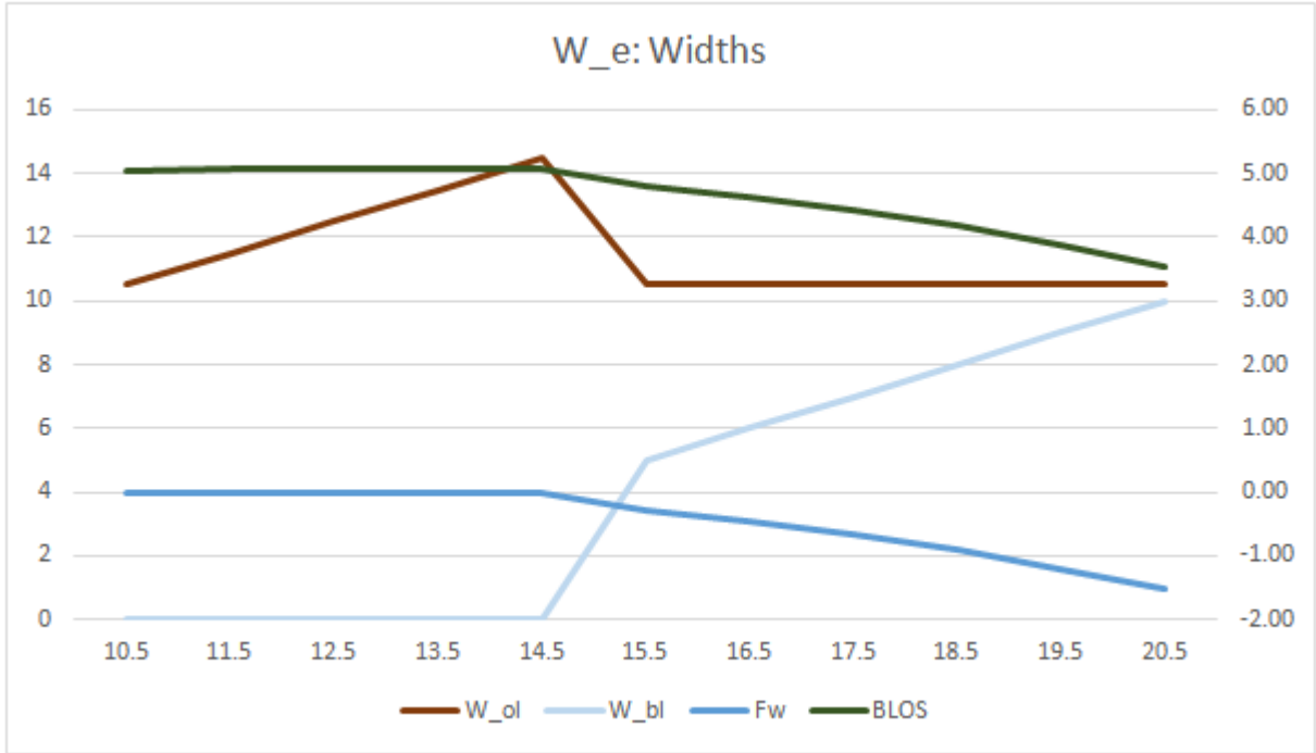
Figure 22: Sensitivity of Link BLOS to variations in bicyclists' operating width.
