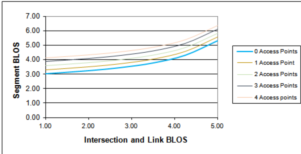
Figure 26: Sensitivity of segment BLOS to the number of right-side access points.
