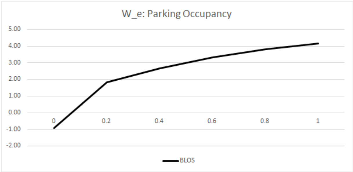
Figure 21: Sensitivity of Link BLOS to variations in parking occupancy
