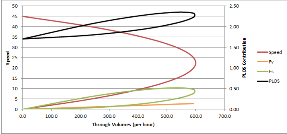
Figure 7: Paradigmatic relationship between traffic speed and traffic flow, or volume, and resulting Intersection PLOS.
