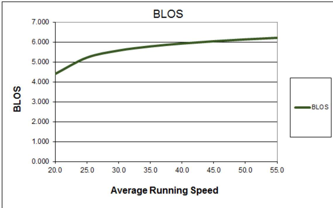
Figure 24: Sensitivity of Link BLOS to variations in vehicle speeds.
