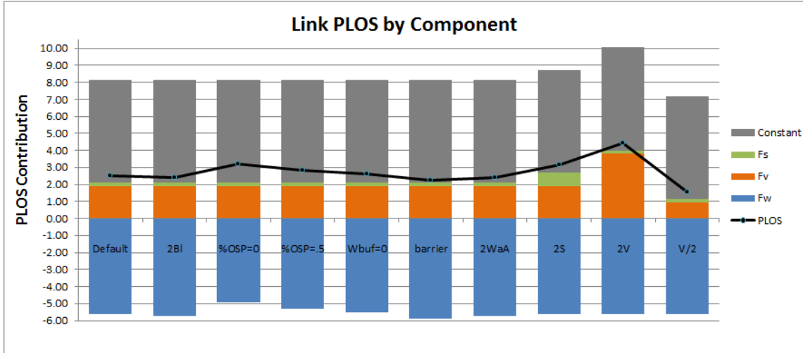
Figure 12: Contributions of F_w , F_v , F_s , and the constant to Link PLOS for a variety of cases.
