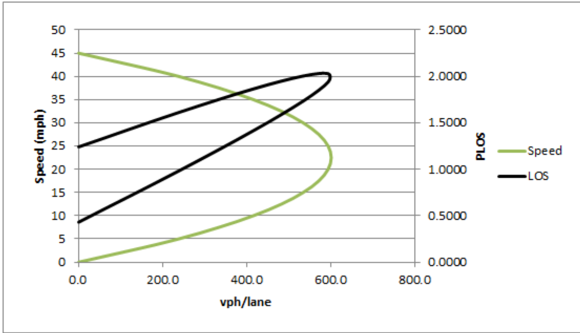
Figure 14: Link PLOS where speed and volume vary according to the fundamental law of traffic engineering.
