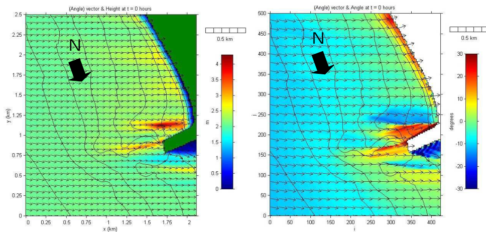
Figure 5-18. Predicted wave height and angle at “The Poles” for a 2 m, 15 s, -10° wave. The true magnetic wave direction is approximately 100°.
