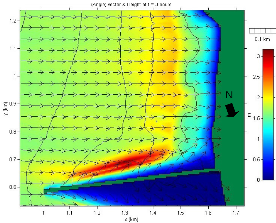
Figure 5-12. Predicted wave height and angle at South Mission Beach for a 1.5 m, 15 s, 0^\circ wave. The true magnetic wave direction is approximately 270^\circ .
