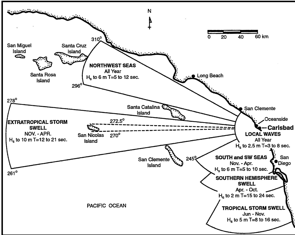
Figure 4-3. Wave exposure for Carlsbad, illustrating island-shadowing effects (from Elwany et al., 1999).
