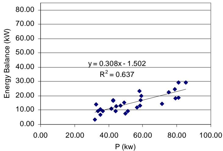
Figure 9.6. Energy Balance Correlation with Compressor Power
