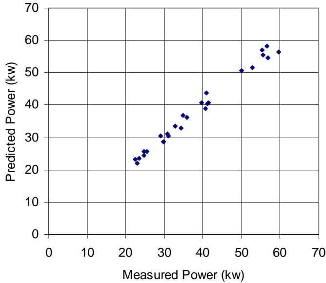
Figure 9.20. Gordon-Ng Model Results - Laboratory Chiller (Adjusted Data)
