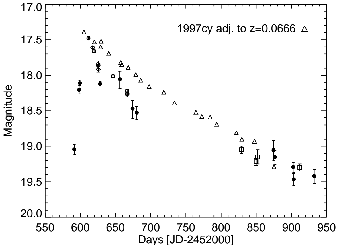
Fig. 4.— The NEAT unfiltered and Hamuy V-band observations of SN 2002ic compared to the K-corrected V-band observations of SN 1997cy from Germany et al. (2000). No date of maximum or magnitude uncertainties are available for SN 1997cy. Here the maximum observed magnitude for SN 1997cy has been adjusted to the redshift of 2002ic, z=0.0666 (Hamuy et al. 2003), and the date of the first light curve point of SN 1997cy has been set to the date of maximum for SN 2002ic from our V-band fit.
