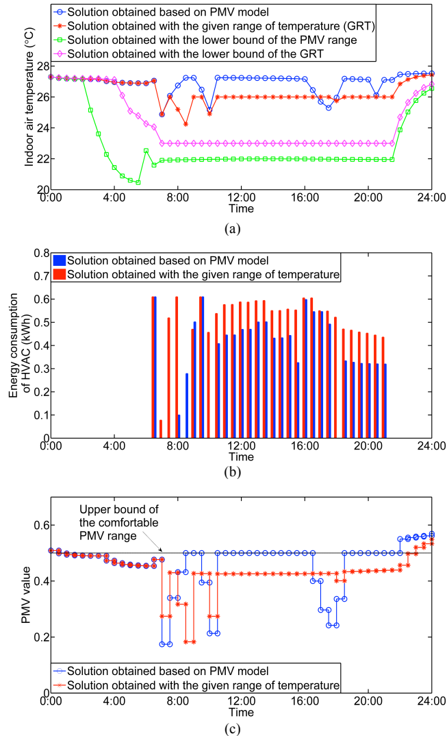
Fig. 7. (a) Comparison of the indoor air temperature; (b) Comparison of the energy consumption of HVAC; (c) Comparison of the PMV values. Note that the energy consumption of the HVAC is the summation of that of the FCU, the DOAS, and other parts of HVAC.
