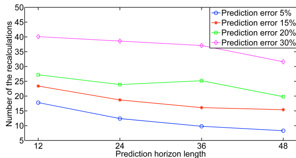
Fig. 9. Computational effort under different combinations of prediction horizon length and prediction error.
