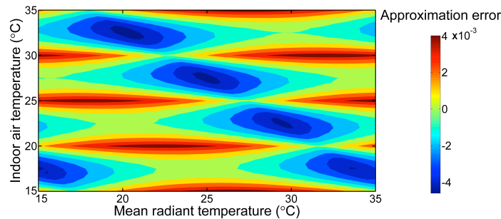
Fig. 2. The error (original PMV-approximate PMV) of the approximation over a temperature range between 15 and 35 °C; air velocity = 0.18 m/s; relative humidity = 55%; metabolic activity = 1.2 met; and clothing insulation = 0.65 clo.
