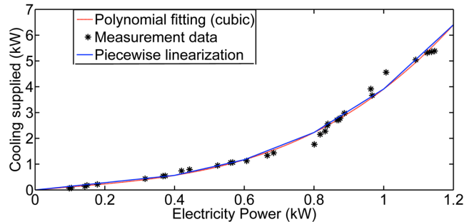
Fig. 5. HVAC model obtained based on the measured data.
