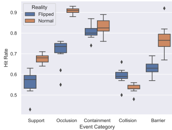
Figure 4: Box plots of Hit Rate for OFPR-Net when trained on only surprising videos (flipped reality) or only expected videos (normal reality) with the outliers shown.
