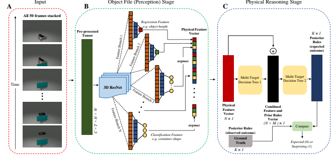
Figure 2: The OFPR-Net architecture. (A) Input: the original data inputs for the VoE task comprise 50 stacked frames. (B) Object File (Perception) Stage: The pre-processed input is fed into a 3D ResNet which then copies its output to N feature branches. Each branch predicts either a scalar or classification feature. (C) Physical Reasoning Stage: The concatenated feature vector is fed into a multi-target decision tree to predict prior rules. The prior rules are concatenated with the feature vector and fed into another multi-target decision tree to predict the posterior rules. The predicted posterior rules are compared with the ground truth to determine if the input scene is surprising .
