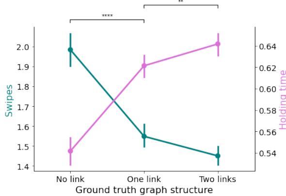
Figure 5: Mean number of swipes performed on a node and mean holding time of each action performed on a node for each case of underlying structure: no link, one link and two outgoing links. All pairwise differences were significant.
