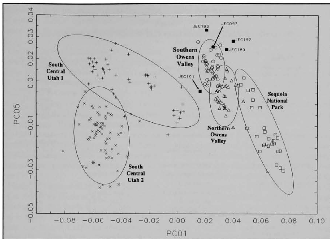
Fig. 3. Plot of principal components of southern Owens Valley, northern Owens Valley, Sequoia National Park, and south-central Utah sherds, showing separation of groups.
