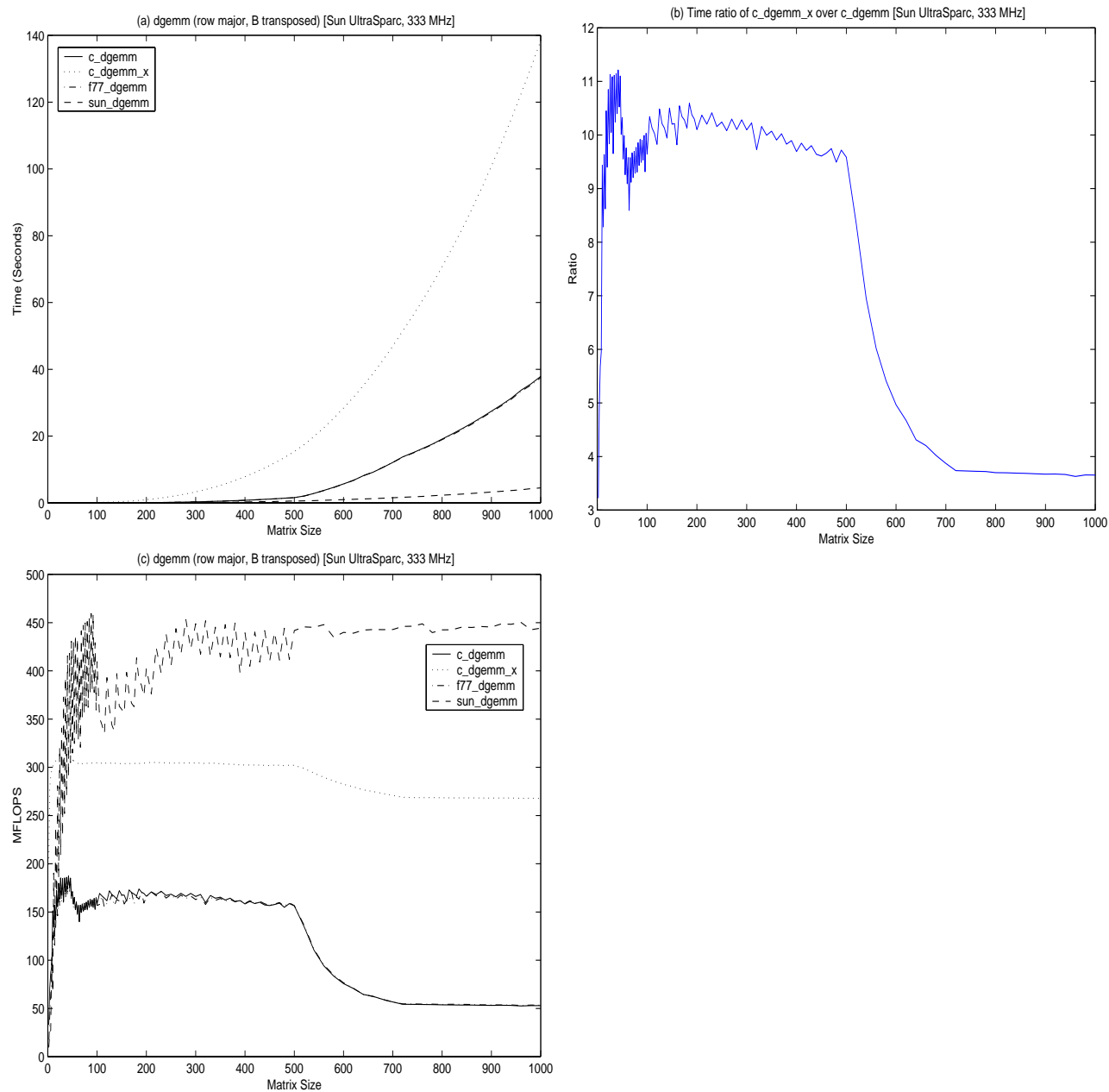
Figure 9: GEMM performance.
