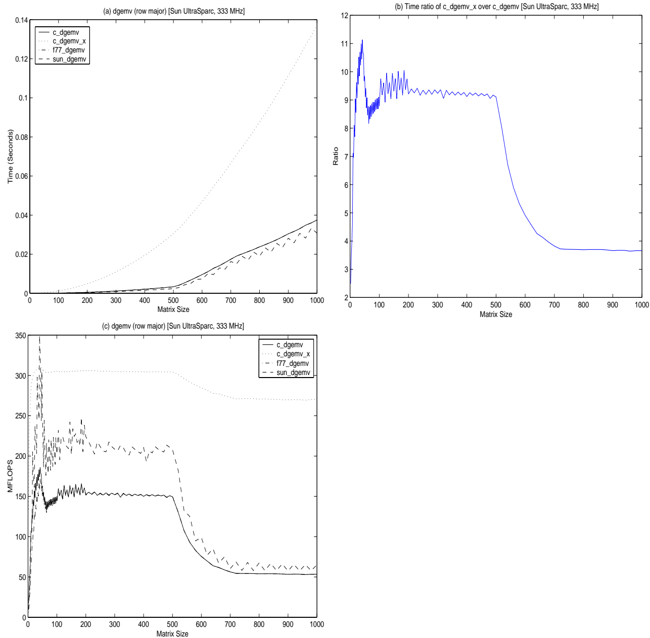
Figure 8: GEMV performance.
