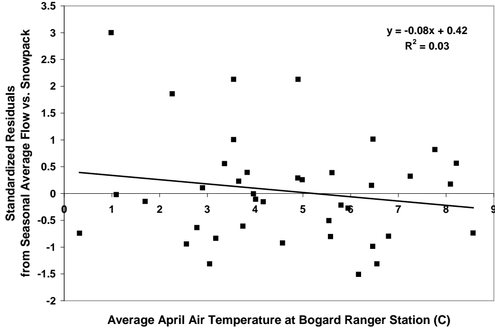
Figure 15. Residuals from regression of seasonal average daily mean streamflow vs. snowpack, plotted against average April air temperature in the upper Pine Creek watershed (data estimated for Bogard Ranger Station COOP site). Data for 1961-1966, 1968, 1970-1981, 1983-1994, 1997-
