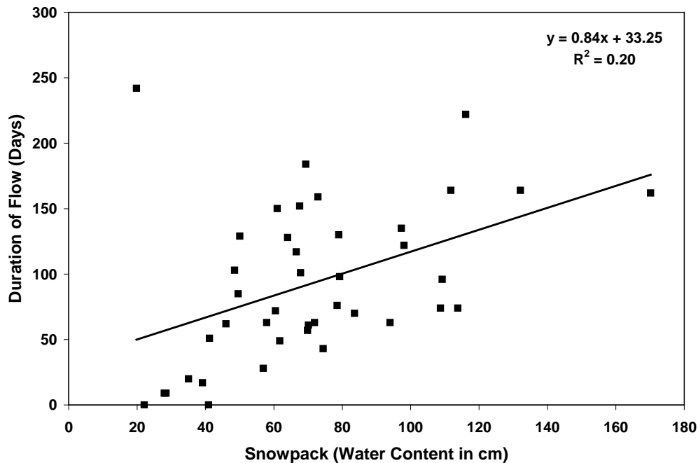
Figure 13. Duration of annual streamflow plotted against April snowpack in the upper Pine Creek watershed (data from Silver Lake site in Susan River watershed). Data for 1961-1966, 1968, 1970-1981, 1983-2004, n=41. Flow data were not collected in 1967 and 1969, or after 2004. Snowpack data were not available for April 1982.
