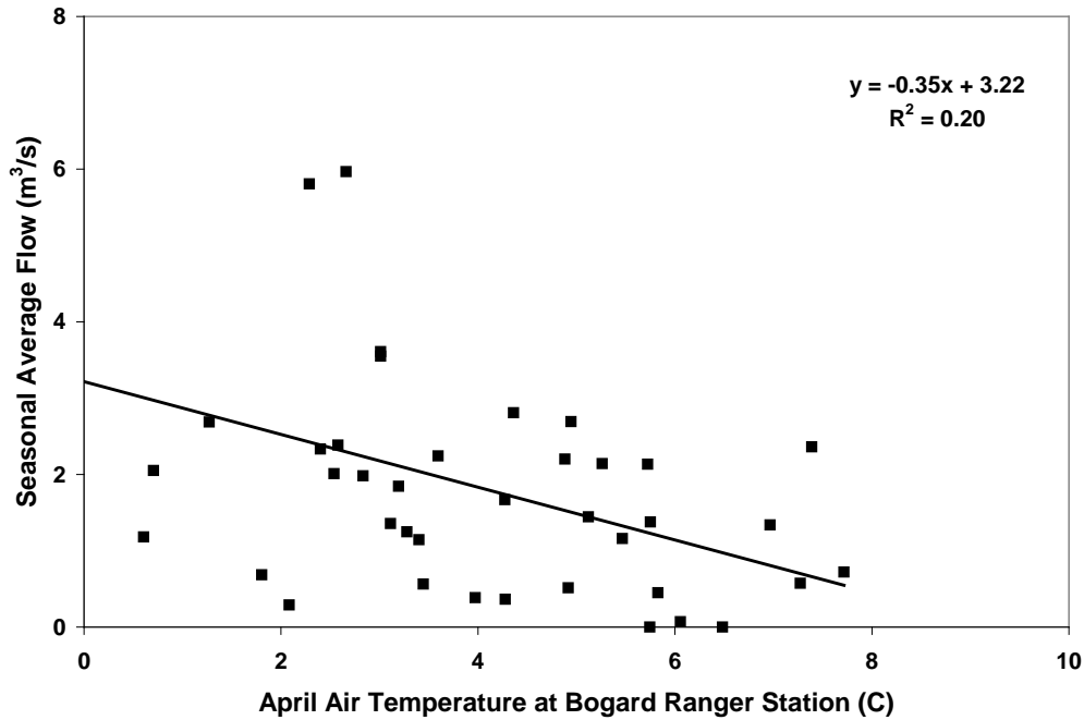
Figure 14. Seasonal average daily mean streamflow plotted against average April air temperature in the upper Pine Creek watershed (data estimated for Bogard Ranger Station COOP site). Data for 1961-1966, 1968, 1970-1994, 1997-2004, n=40. Flow data were not collected in 1967 and 1969, or after 2004. Air temperature data were not available for 1995 and 1996.
