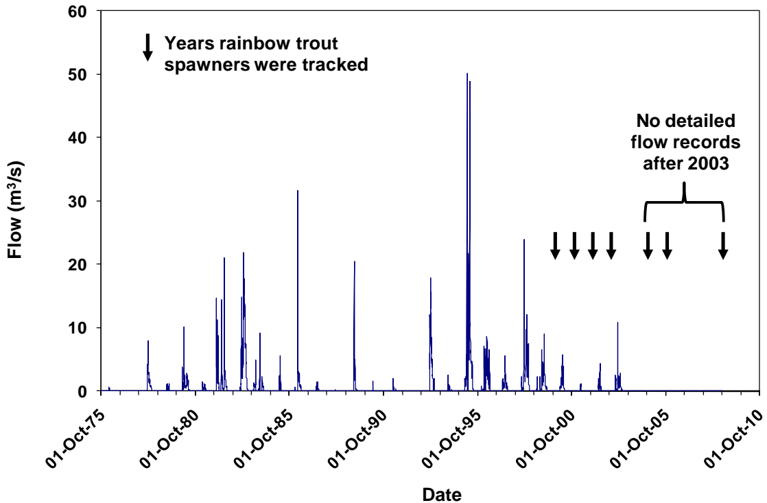
Figure 7. Mean daily streamflow for DWR gage G31140, near the mouth of Pine Creek, and years in which rainbow trout spawner migration was tracked. Flow data courtesy of John Clements, DWR.
