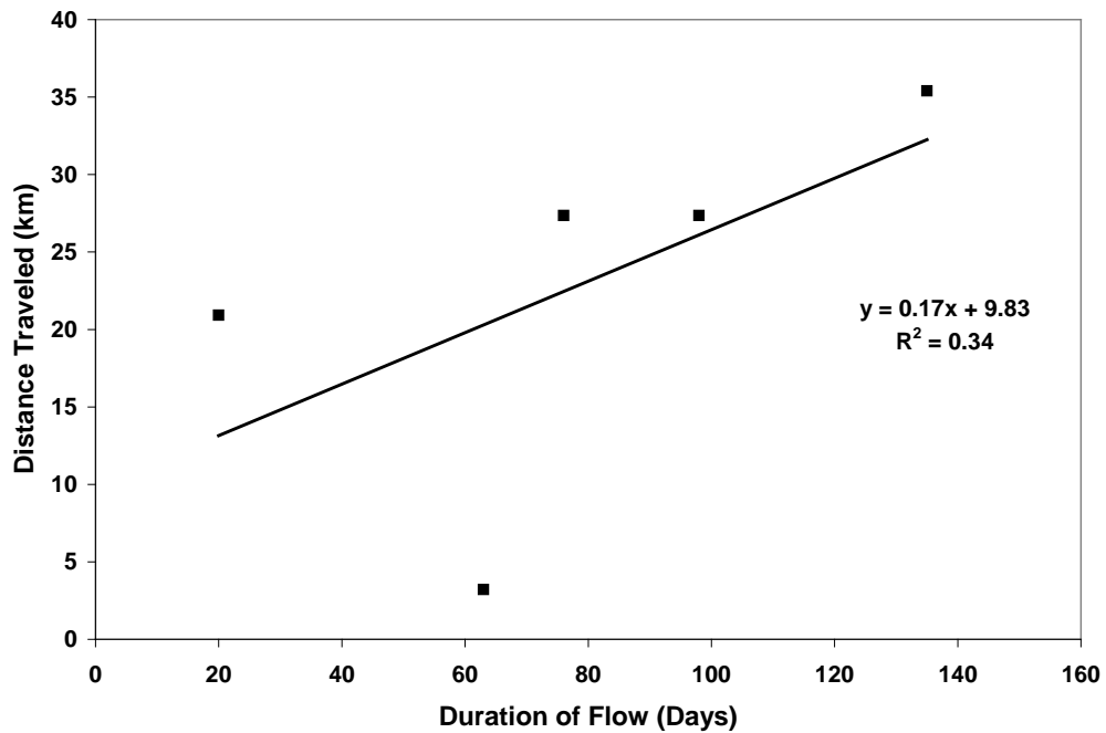
Figure 9. Maximum distance that a rainbow trout migrated upstream plotted against duration of streamflow for that year. Data for 1999-2002, 2004; n, n=5.
