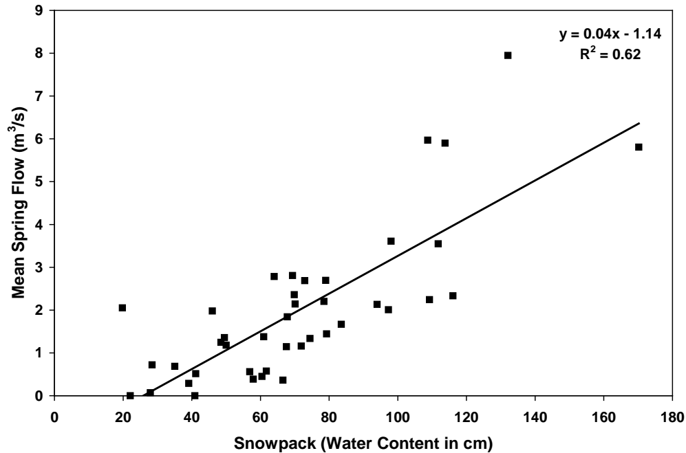
Figure 12. Seasonal average daily mean streamflow plotted against April snowpack in the upper Pine Creek watershed (data from Silver Lake site in Susan River watershed). Data for 1961-1966, 1968, 1970-1981, 1983-2004, n=41. Flow data were not collected in 1967 and 1969, or after 2004. Snowpack data were not available for April 1982.
