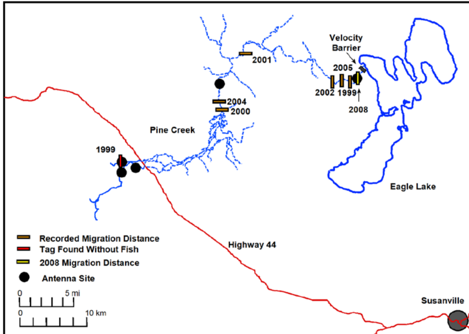
Figure 1. Map of Eagle Lake and Pine Creek, showing passive integrated transponder antenna sites (2008) and maximum distance that rainbow trout spawners migrated in each year. Note: Migration distances indicated by marks are approximate; marks were shifted to avoid overlap. Accurate distances are given in Table 1.
