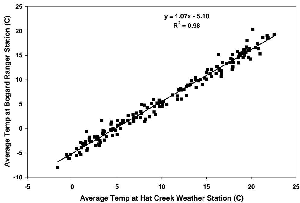
Figure 5. Comparison of mean monthly air temperature at Bogard Ranger Station RAWS site and Hat Creek PH 1 COOP site, from 1992-2008. n=170.
