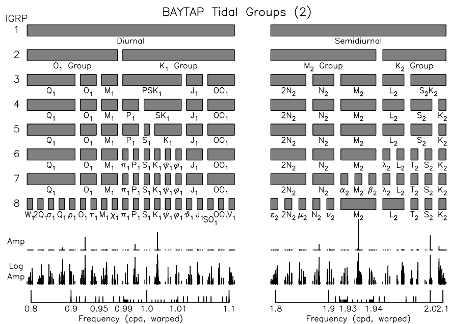
Figure 2: Diurnal and semidiurnal tidal groups available with the default option in Baytap, shown with the frequency axis warped to make each of the groups (in the finest subdivision) equal in size; the ticks at the bottom are for 0.1, 0.01, and 0.001 cycles/day, chosen to avoid crowding. The two lines below the groups show the amplitude spectrum of tidal harmonics, in both linear and log amplitude.
