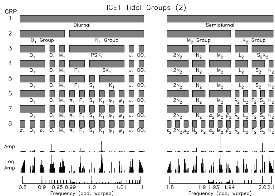
Figure 4: Diurnal and semidiurnal tidal groups available with the icetgr=2 option in baytap08 , shown with the frequency axis warped to make each of the groups (in the finest subdivision) equal in size; the ticks at the bottom are for 0.1, 0.01, and 0.001 cycles/day, chosen to avoid crowding. The two lines below the groups show the amplitude spectrum of tidal harmonics, in both linear and log amplitude.
