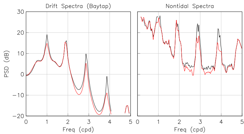
Figure 8: Spectra of the drift and nontidal data from Patricia Bay. Red is after fitting the extra sinusoids.
