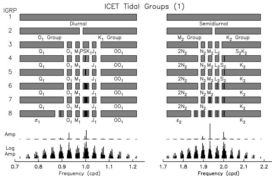
Figure 3: Diurnal and semidiurnal tidal groups available with the icetgr=2 option in baytap08 , shown on a linear frequency axis. Labels omitted if they would overlap. The two lines below the groups show the amplitude spectrum of tidal harmonics, in both linear and log amplitude.
