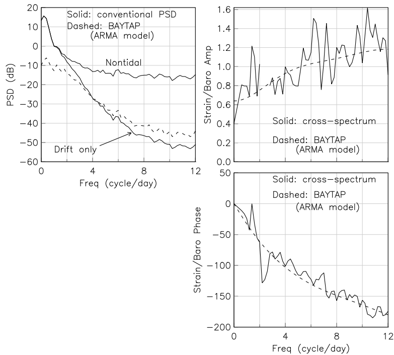
Figure 6: Spectra of the drift and nontidal data from Esashi, and the transfer function from air pressure to strain.
