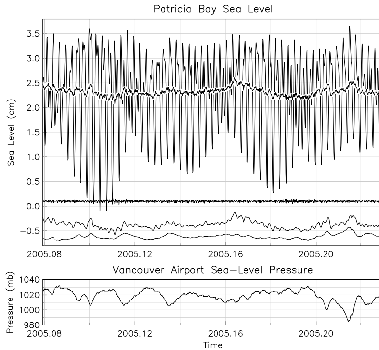
Figure 7: Sea-level data from Patricia Bay, Canada (adjacent to the Pacific Geoscience Center) as processed by baytap08
