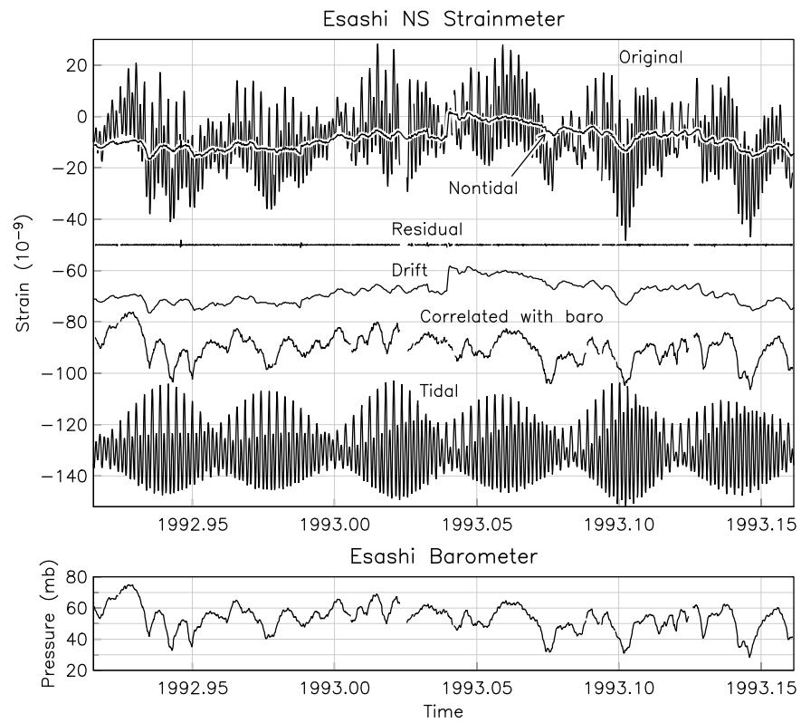
Figure 5: Strainmeter data from Esashi, Japan, as processed by baytap08
