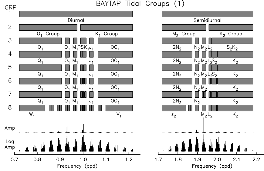
Figure 1: Diurnal and semidiurnal tidal groups available with the default option in Baytap, shown on a linear frequency axis. Labels omitted if they would overlap. The two lines below the groups show the amplitude spectrum of tidal harmonics, in both linear and log amplitude.
