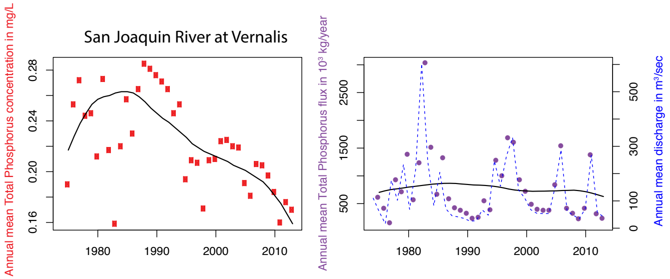
Figure 11 TP concentration and flux at the outlet of the San Joaquin River at Vernalis site. Annual mean concentrations of TP (solid red dots), annual total load of TP (purple dots), annual mean discharge (dashed blue line), and flow normalized trends (solid black lines) are shown.
