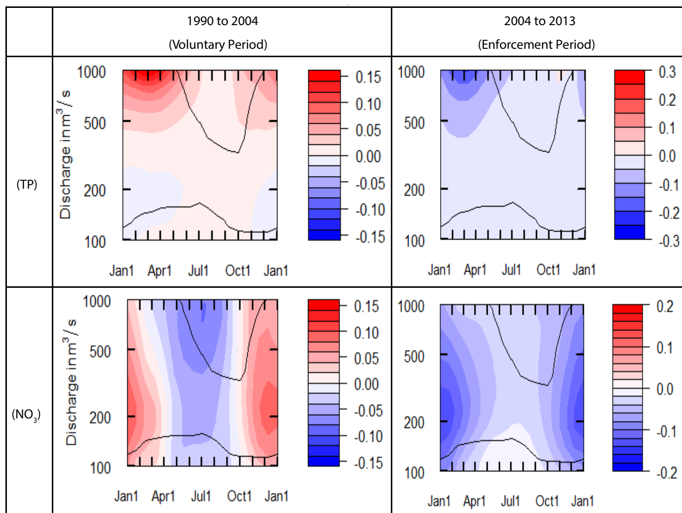
Figure 9 Estimated changes in concentrations of TP (A) and NO 3 (B) from 1990 to 2004 (left column plots) and 2004 to 2013 (right column plots) for the Sacramento River at Colusa site. The upper and lower solid black lines represent the 95% and 5% percentiles of flows. Months are shown on the X-axis and integrate all data for the time period shown. Red indicates increasing concentrations and blue indicates decreasing concentrations.
