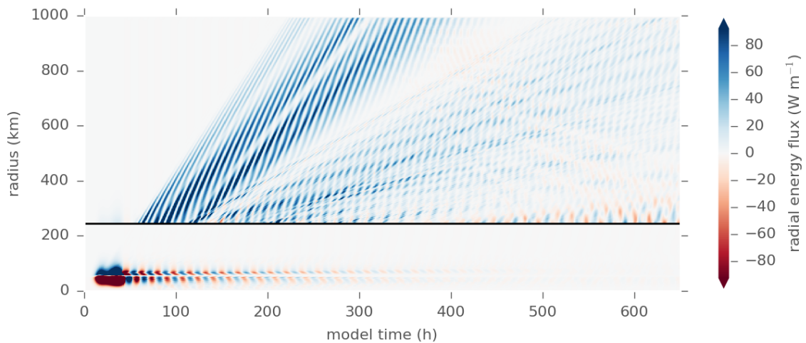
Figure 4: Largest value of the azimuthally integrated radial energy flux 2\pi R(u'p') throughout the water column with MLD = 500 m. The black line marks the border between near and far field. The colorbar corresponds to the far field.
