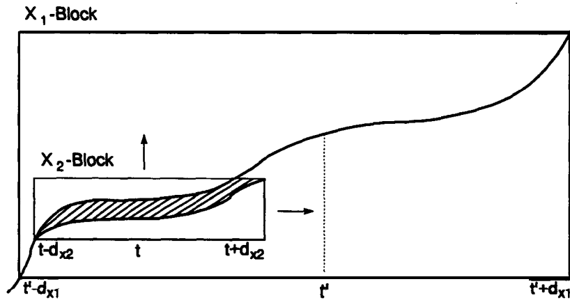
Figure 2.4 Least squares method applied to correlate parts of the cumulative curves \alpha_{x_1}(t) and a_2(t)
