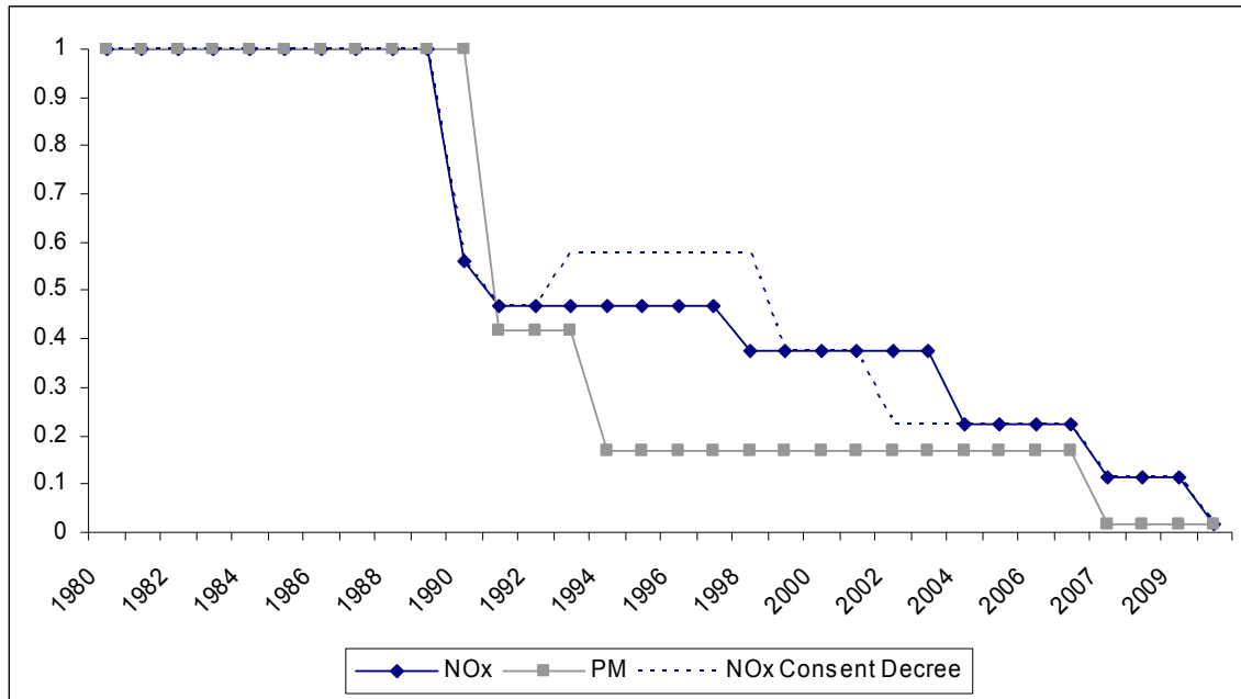
Figure 1: Proportional Declines in Federal NOx and PM Diesel Engine Emissions Limits (1980-2010) 14
