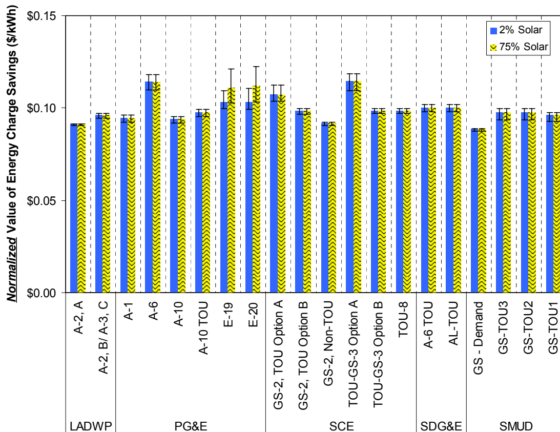
Figure 22. Normalized Value of Energy Charge Savings
