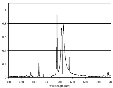
HPS (2500 K)
