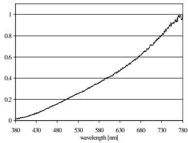
Incandescent (2850 K)
