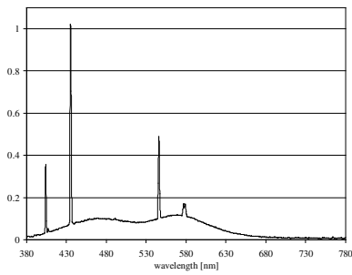
Fluorescent –T12 (6500)
