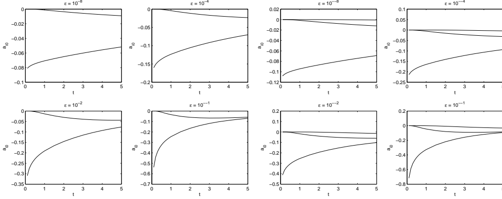
FIGURE 5. Coefficients a_{i0}(t) for rectangles with a = 2 , b = 1 . Left four panels: three rectangles ( N = 2 ) with (Y_1, Y_2) = (0.3, 0.9) ; right four panels: four rectangles ( N = 3 ) with (Y_1, Y_2, Y_3) = (0.3, 0.9, 0.2) .
