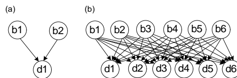
Figure 2: Causal networks generated by grammar G_3 after (a) phase 0 and (b) phase 3 of the experiment.
