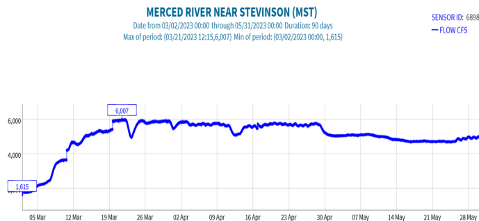
Figure 6. Hourly River Flow — March to May 2023 (MST Station) Sustained high flows linked to prolonged snowmelt and dam control.
