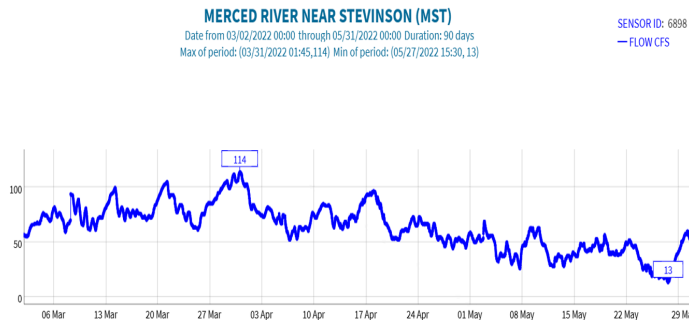
Figure 5. Hourly River Flow — March to May 2022 (MST Station) Sharp peak and steep drop reflect rapid, unregulated melt.
