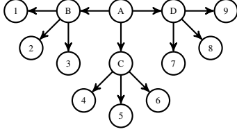
Figure 3: The ‘Big net’ from base NormAN, featuring hypothesis A, and evidence nodes 1 through 9, of which the first three correlate with the hypothesis, the last three anti-correlate, and the middle three are non-diagnostic.
