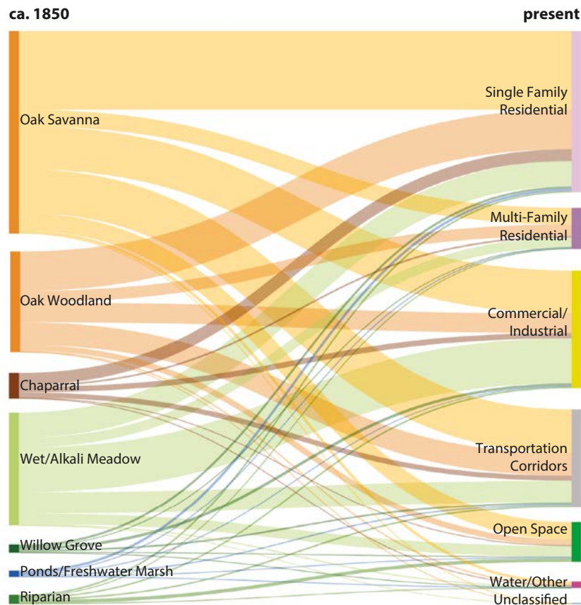
Land cover/land use transformation in Santa Clara Valley, ca. 1850 to present day (ca. 2013). The thickness of each line corresponds to the total area that has undergone each transformation.
