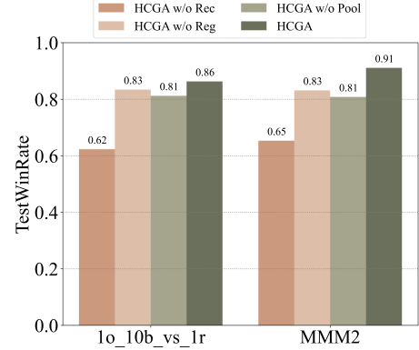
Figure 4: Ablation studies of HCGA modules.
