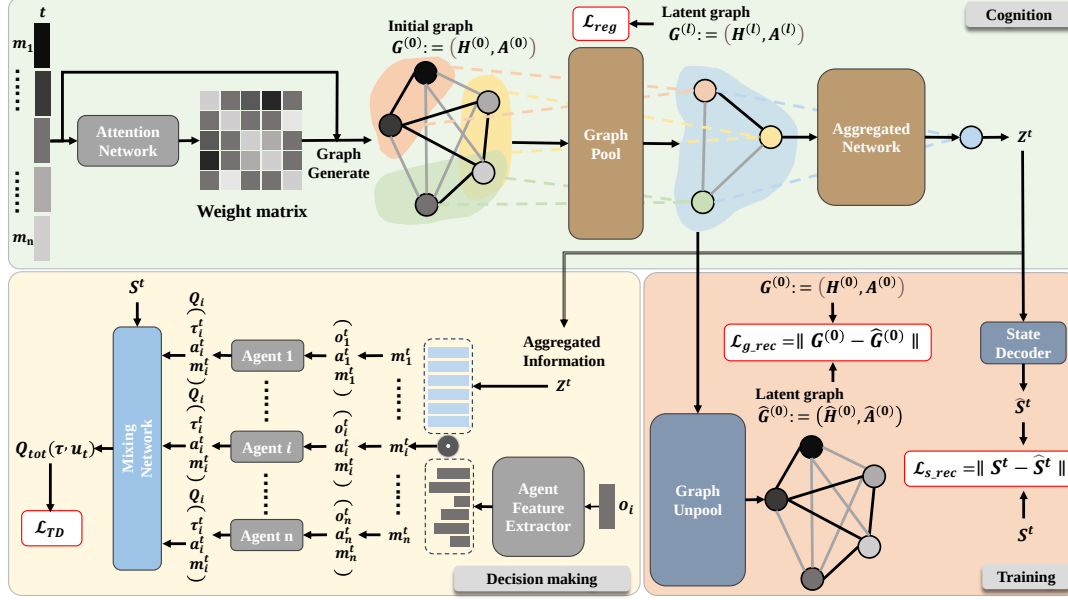
Figure 2: The HCGA framework consists of three modules: cognition, training, and decision making. The cognition module constructs a weighted communication graph via attention and pools it into a latent graph for global representation. The training module refines information through graph unpooling and state reconstruction. In the decision-making module, agents extract personalized features from the aggregated representation to guide their actions.
