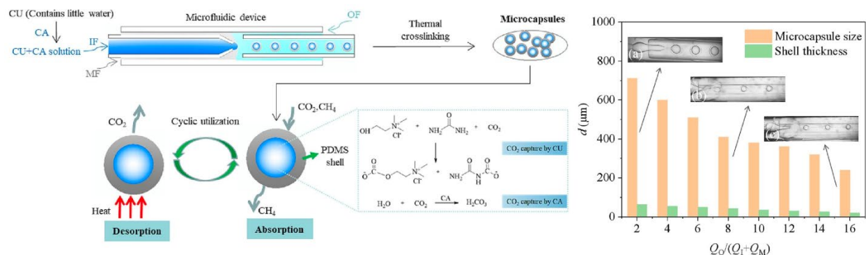
Figure 3. [Left] Schematic diagram of the flow-focusing microchannel, encapsulating DES and CA. IF-Inner Fluid; MF-Middle Fluid; OF-Outer Fluid. [Right] Effect of the flow rates on the microcapsule size and shell thickness in a 3D glass-capillary microfluidic device. (In the graph; “d” as a function of Q_O/(Q_I + Q_M) - flow rate of inner fluid; Q_M - flow rate of middle fluid; Q_O - flow rate of outer fluid.). 31
