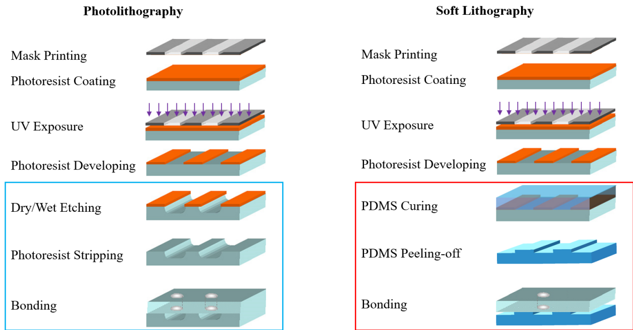
Figure 21. [Left] Major fabrication steps carried out for photolithography and [Right] soft lithography. While both methods start with mask making and photoresist processing, photolithography typically finishes with etching and bonding of silicon and/or glass, but soft lithography finishes with PDMS molding.
