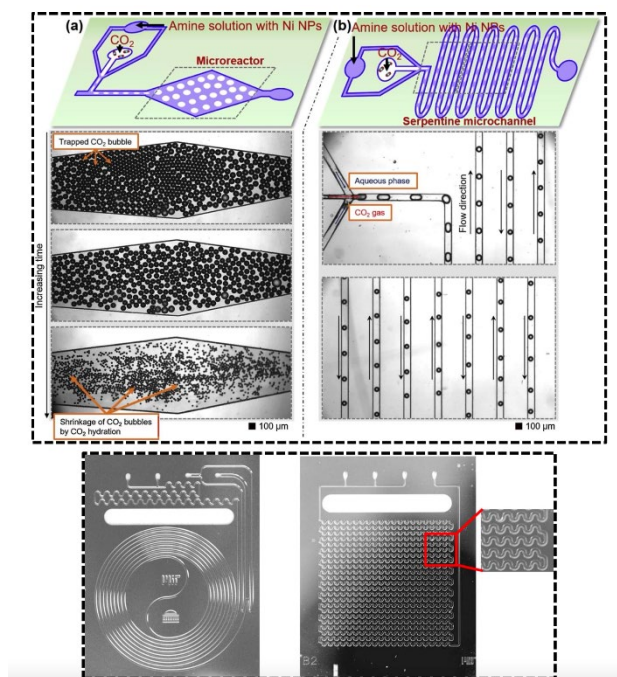
Figure 15. [Top] Schematic of the microfluidic approaches for evaluating CO 2 absorption. The top panel illustrates two designs. (a) Microreactor operating under limited mixing conditions, along with sequential images showing changes in CO 2 microbubble size. (b) A long serpentine microchannel under high mixing conditions, with images of CO 2 microbubbles at two different locations. The scale bar represents 100 μm 81 . [Bottom] Actual photograph of the spiral channel and meandering channel geometries. 80
