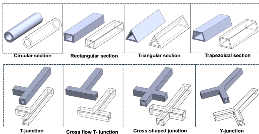
Figure 13. Illustration of different cross sections of microchannels, different junctions in microchannel geometries, and their wireframe views.
