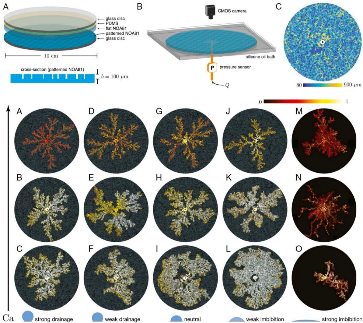
Figure 27. [Top] schematic showing the micromodel used for the study of wettability effects by Zhao et al. (2016); the micromodel was made of a photocurable polymer (NOA81) patterned with circular posts; [Bottom] displacement patterns for various wettability conditions (left to right: \theta = 150^\circ, 120^\circ, 90^\circ, 60^\circ, 7^\circ ) and capillary numbers (bottom to top: Ca = 2.9 \times 10^{-3}, 2.9 \times 10^{-2}, 2.9 \times 10^{-1} ).
