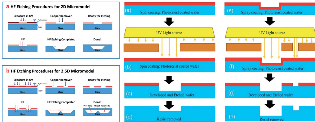
Figure 22. [Left] Fabrication steps of a 2.5D micromodel. 173 [Right] Fabrication steps of a dual-porosity dual-depth micromodel. 181
