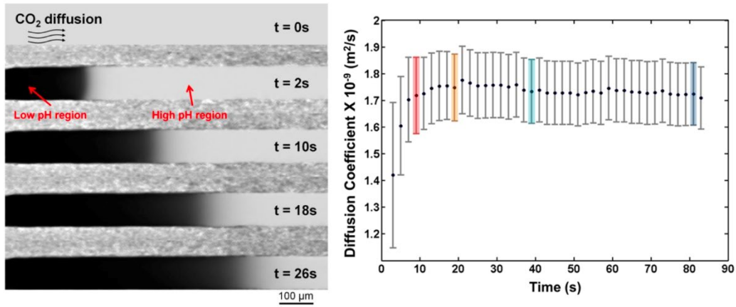
Figure 7. [left] Visualization and analysis of \text{CO}_2 diffusion into water. Time-lapse images showing fluorescent quenching as \text{CO}_2 diffuses into water, leading to solution acidification. Diffusion coefficients were obtained at a pressure of 5 bars. A diffusion coefficient is determined for each frame captured during the experiment, with each data point spaced 2 s apart. The error bars account for uncertainties in measurements (e.g., initial pH, temperature) and their effect on the calculated diffusion coefficient ( D ). [Right] The overall diffusion coefficient at this pressure is determined as D = 1.74 \times 10^{-9} \text{ m}^2/\text{s} , obtained by averaging individual D values. 49
