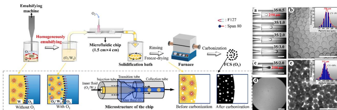
Figure 4. [Left] Illustrative image of the fabrication of microporous carbon spheres. [Right] (a) Experimental images showing the controllable formation of emulsions at varying flow rates (values in each photo indicate the outer-to-inner phase ratio), (b) Optical micrographs of solidified 2% FS with an inset displaying the particle size distribution, (c) Formation of double emulsions, (d) Optical micrographs of nanodroplets dispersed in water, and (e) Optical micrographs of solidified 2% FS with 10% oil phase, with insets showing the corresponding particle size distributions. Scale bars: 1000 μm. 44
