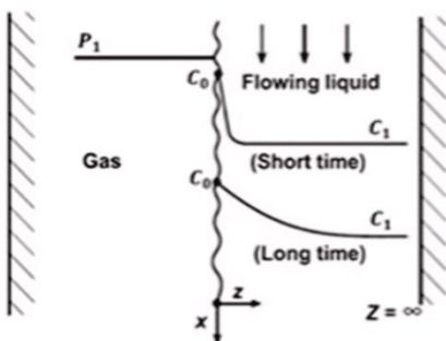
Figure 12. Illustrative image showing gas-liquid interaction representing penetration mass transfer theory. 62
