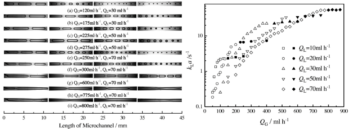
Figure 11. [Left] Experimental image of gas-liquid flow at different flow rates. [Right] The calculated volumetric mass transfer coefficient ( k_{La} ) for different flow rates. 58
