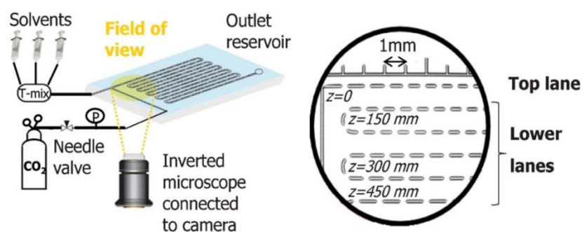
Figure 2. Schematic representation of the experimental setup with the Field of view. In the field of view, the top lane shows bubble shrinkage due to absorption, lower lanes, and slow expansion due to pressure drop. 29
