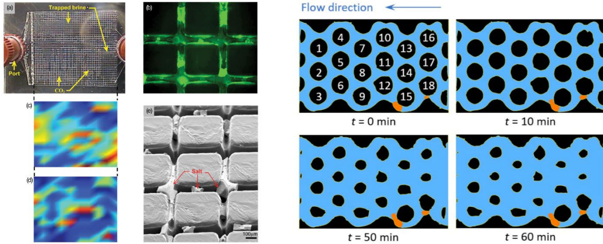
Figure 29. [Left] Experiments of salt precipitation in the regular grid-like microfluidic network in PMMA. 192 [Right] evolution of the calcite grains over time subject to dissolution by HCl. The dissolution rate is shown to be strongly dependent on the pore flow and the presence of gas bubbles. 187
