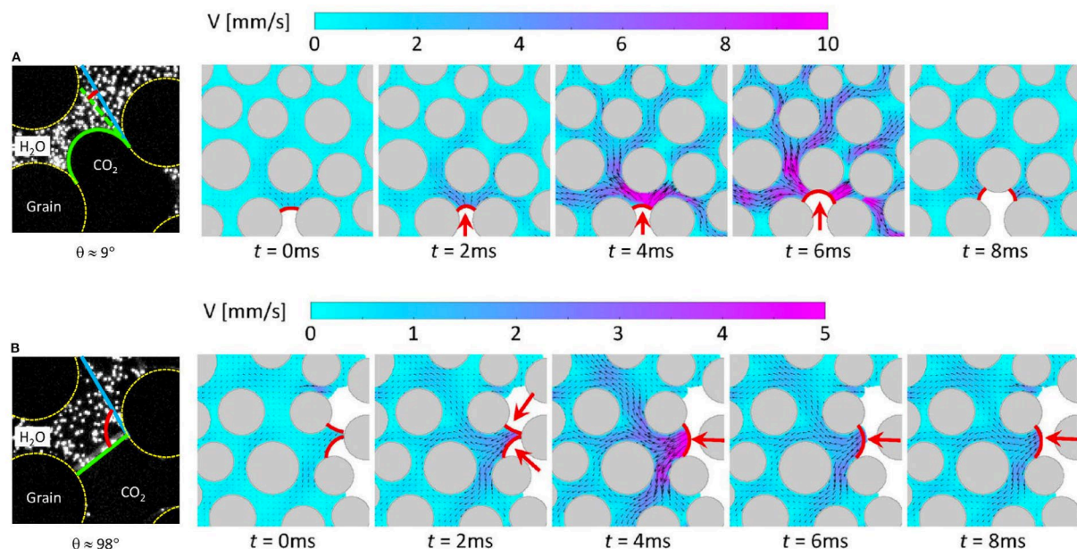
Figure 28. [Top] Evolution of velocity fields during a Haines jump event in drainage. [Bottom] Evolution of velocity fields during a cooperative filling event in weak imbibition. 166
