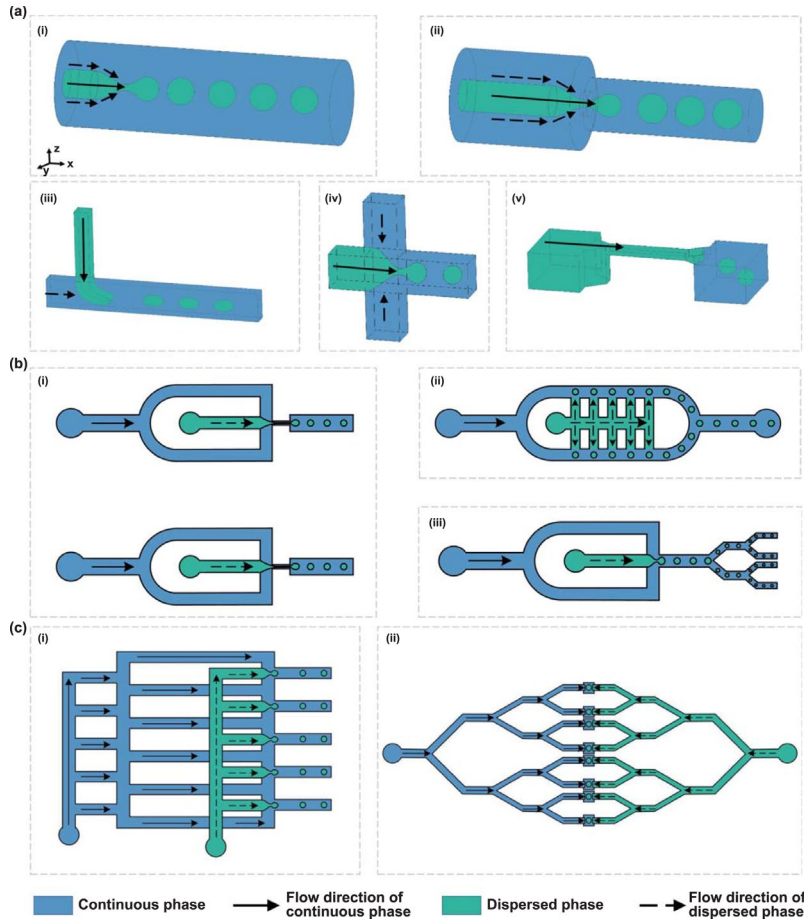
Figure 14. Schematic illustration of microchannel characteristics. (a) Flow behaviors in different droplet generators: (i) co-flow, (ii) flow-focusing, (iii) T-junction, (iv) cross-junction, and (v) step emulsification, demonstrating various methods for generating emulsions in microfluidic systems. (b) The scale-up strategies for microfluidic processes: (i) parallel numbering-up of both dispersed and continuous phase nozzles, (ii) parallel numbering-up of dispersed phase nozzles only, and (iii) splitting of emulsion droplets to achieve higher throughput. (c) The fluids distribution network in two common layouts: (i) ladder network and (ii) tree network, illustrating different methods for ensuring uniform flow distribution across multiple microchannels. 18
