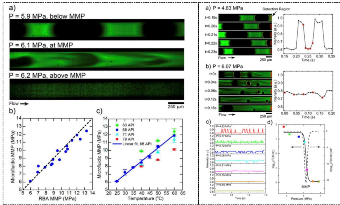
Figure 17. Fluorescence-based microfluidic measurement of MMP for CO 2 in crude oils. (a) Fluorescence images of CO 2 bubbles at different pressures: below MMP (5.9 MPa), at MMP (6.1 MPa), and above MMP (6.2 MPa), showing the transition from distinct CO 2 bubbles to complete mixing. (b) Correlation between microfluidic MMP measurements and rising bubble apparatus (RBA) MMP values showing strong agreement. (c) Temperature dependence of MMP for synthetic oil mixtures of varying API gravities, demonstrating a linear increase in MMP with temperature. (d) Automated fluorescence intensity analysis for different pressures, with fluorescence fluctuations decreasing above MMP, enabling precise determination of MMP via intensity variance analysis. 85
