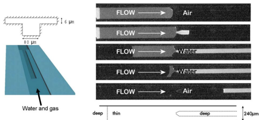
Figure 18. [Left] Microfluidic gas-liquid phase separation for \text{CO}_2 measurement. Schematic of the microchannel design, featuring deep and thin regions for controlled phase separation. [Right] Experimental images showing sequential air and water flow, demonstrating effective gas isolation for inline \text{CO}_2 analysis with infrared absorption spectroscopy. 86
