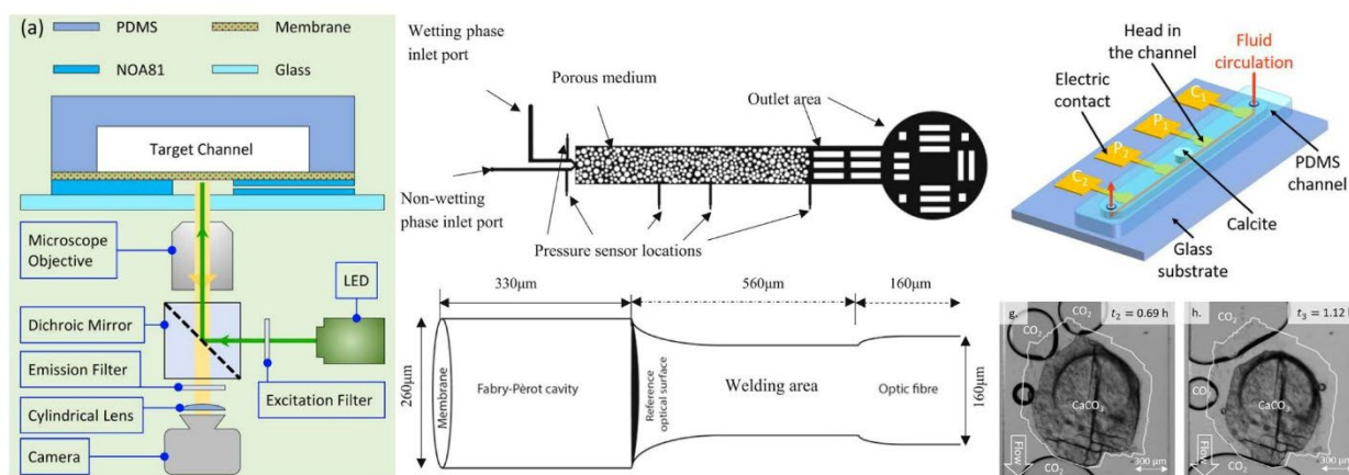
Figure 24. [Left] A schematic diagram illustrating the on-chip pressure sensor enabled by astigmatic particle tracking. 191 [Middle] Micromodel with integrated fiber optical pressure sensors. 190 [Right] 3D sketch of the microfluidic chip with integrated SIP sensors and sample results of calcite dissolution. 189
