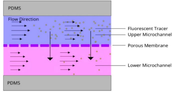
Figure 9. Schematic representation of convection-diffusion mass transport in a microfluidic device. Molecules from the high-concentration stream (purple) diffuse into the low-concentration stream (pink) while convecting downstream, illustrating the simultaneous influence of advection and diffusion on mass transfer within the microchannel. 52
