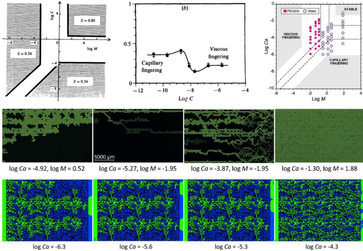
Figure 25. [Top Left]: the original phase diagram achieved by Lenormand et al., demonstrating the existence of capillary fingering, viscous fingering, stable displacement regimes, and the crossover between them. 131 [Top Middle]: plot of the invading fluid at breakthrough, showing a decrease of the nonwetting phase saturation at the crossover between capillary and viscous fingering. 131 [Top Right]: an updated phase diagram obtained by Zhang et al. 140 [Middle Row] Representative displacement patterns for capillary fingering, crossover, viscous fingering, and stable displacement, respectively, captured in homogeneous micromodels. 140 [Bottom Row] Representative displacement patterns going from capillary fingering to crossover, and finally to viscous fingering as the capillary number increases in 2D heterogeneous micromodels. 137
