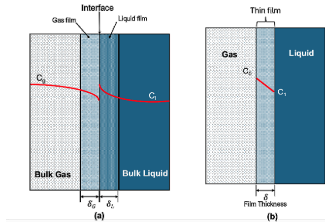
Figure 10. Illustrative images of mass transfer models, (a) Two film mass transfer, (b) Thin film mass transfer.
