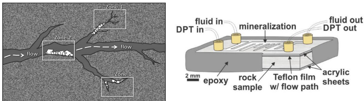
Figure 19. [Left] The schematic of carbon mineralization occurring in different zones of a fractured mafic/ultramafic rock. [Right] The schematic showing a microfluidic model system used to investigate carbon mineralization in a fracture. 106
