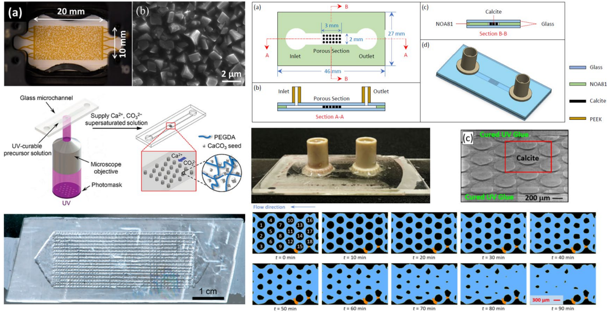
Figure 23. A few representative micromodels that are chemically reactive. [Top left] Hybrid calcite-glass micromodel employing glass etching and in-situ growth of calcium carbonate nanocrystals. 186 [Middle left] A calcite micromodel fabricated using the site-selective in-situ grown calcium carbonate approach. 185 [Bottom left] A calcite micromodel created from a thin slice of calcite employing a laser cutter and wet etching. 178 [Right] Pure calcite micromodel fabricated with photolithography and wet etching. 187
