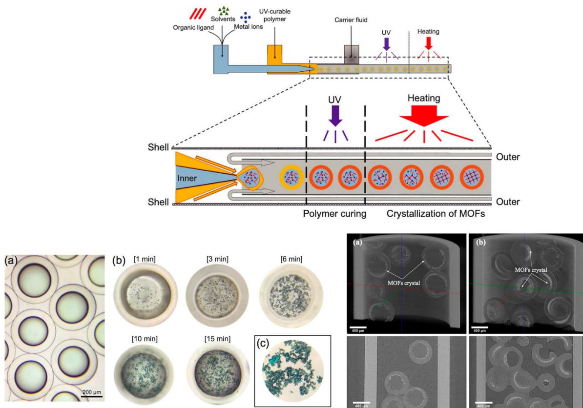
Figure 6. [Top] Schematic representation of the microfluidic system used for the in-situ encapsulated synthesis of MOFs, where the shell material TEGO Rad 2650 is structurally similar to TEGO Rad 2100 and TEGO Rad 2500. [Bottom Left] Microscopic images of encapsulated HKUST-1 crystals: (a) Microcapsules containing precursor solutions of copper(II) nitrate trihydrate ( \text{Cu}(\text{NO}_3)_2 \cdot 3\text{H}_2\text{O} ) and 1,3,5-benzenetricarboxylic acid ( \text{H}_3\text{BTC} ) dissolved in N,N -dimethylformamide (DMF) before heating, (b) Sequential stages of HKUST-1 crystal formation during the in-situ thermal reaction within the microcapsules over a reaction time of 1–15 minutes, and (c) HKUST-1 crystals synthesized via the conventional solvothermal method in bulk solution for comparison; [Bottom Right] Three-dimensional X-ray microtomography of encapsulated HKUST-1 within a glass tube: (a) Microcapsules containing HKUST-1 and residual DMF solvent, and (b) Dried microcapsules after solvent removal. 47
