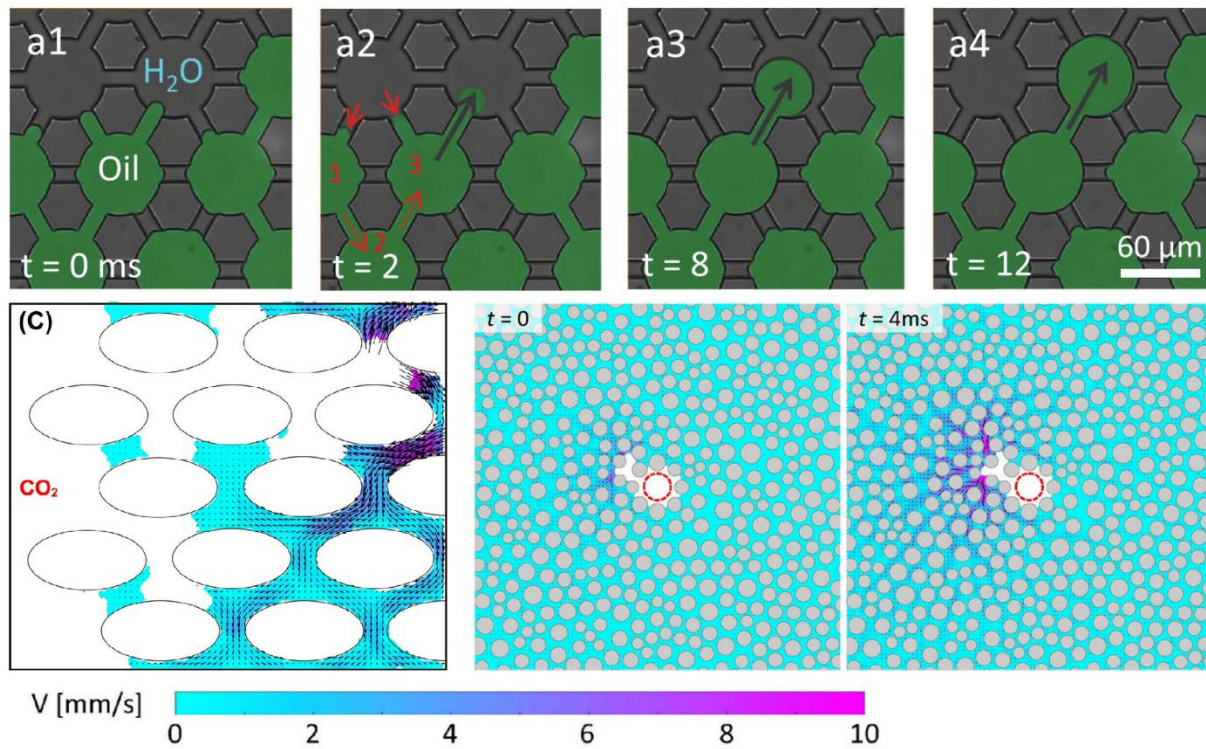
Figure 26. [Top] High speed images of a Haines jump event at Ca = 3.4 \times 10^{-6} . 149 [Bottom] Velocity vector fields during a Haines jump event in linear drainage and radial drainage. 151,157
