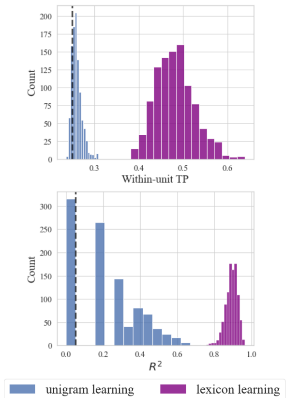
Figure 2: Distribution of mean within-unit transitional probability (top) and R^2 values (bottom), of the 1000 simulated chains after 10 generations. The mean value of generation zero (which is randomly generated) is indicated with the black dashed line.
