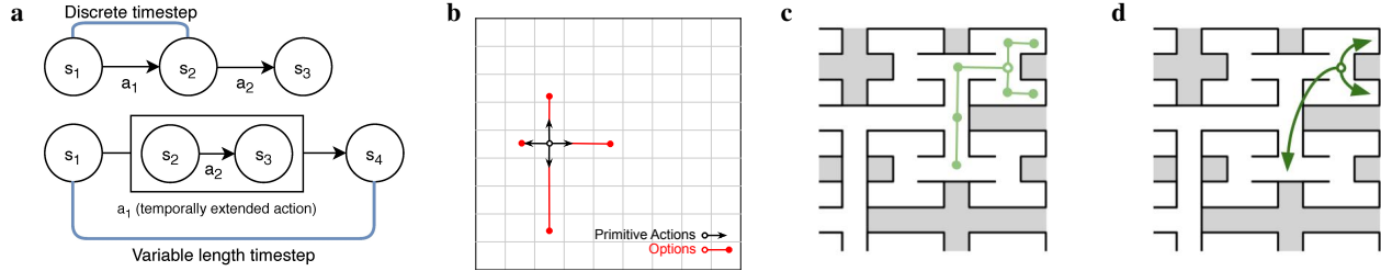
Figure 2: Algorithmic implementation of \epsilon z -greedy in the maze task. (a) The semi-MDP framework (bottom) allows the length between timesteps to be variable in comparison to standard MDP (top) and as such can support temporally extended actions. (b) The set of primitive actions (black) and few possible temporally-extended actions, or options, of variable length timesteps (red) shown for an open grid world environment. Open circle denotes the state where an option is initiated and the solid circle denotes its termination. (c) In the given maze, if modeled as MDP, the agent will only make progress by one node before having to make a decision again at every intermediate turn in the maze. (d) In \epsilon z -greedy model, which is based on the semi-MDP framework, the agent first chooses a direction at random and samples an entire action-sequence and executes it in one go, abstracting away the decisions at intermediate timesteps.
