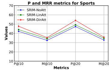
Figure 5: Evaluation of self-attention settings
