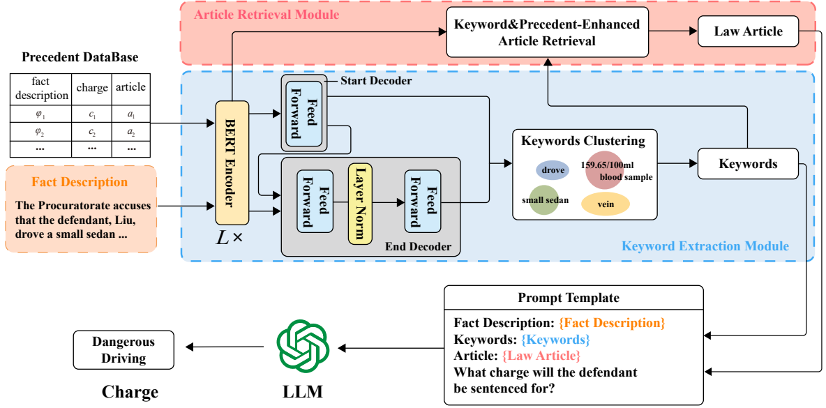
Figure 2: Illustration of our proposed KnowJude framework. KnowJude is composed of two modules: Keyword Extraction Module and Article Retrieval Module.
