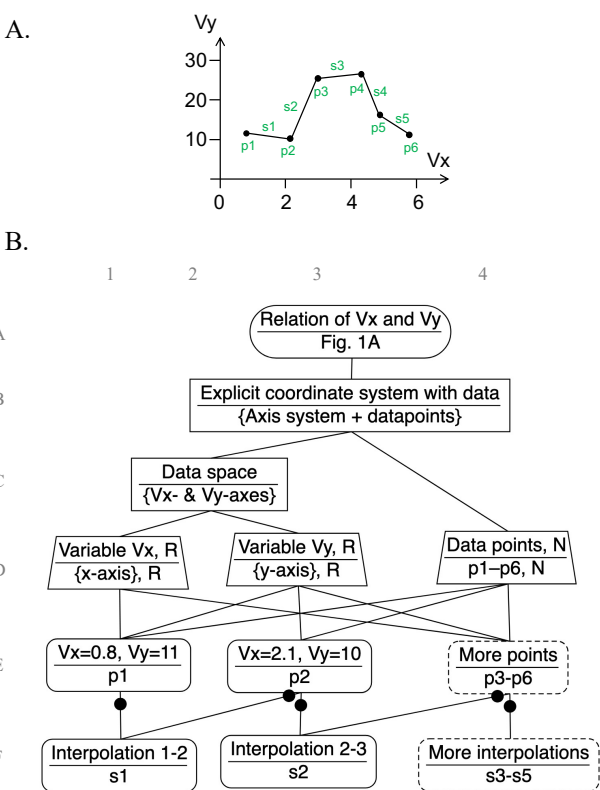
Figure 1. (A) A simple line graph; (B) The RISN model of the interpretation of (A).
