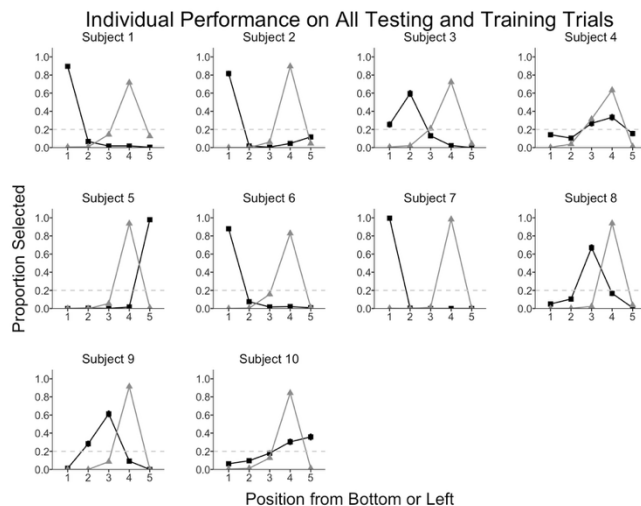
Figure 4: Individual performance on all testing trials (squares) and training trials (triangles). Error bars represent standard error of the mean. Dotted line represents chance levels of 20%.
