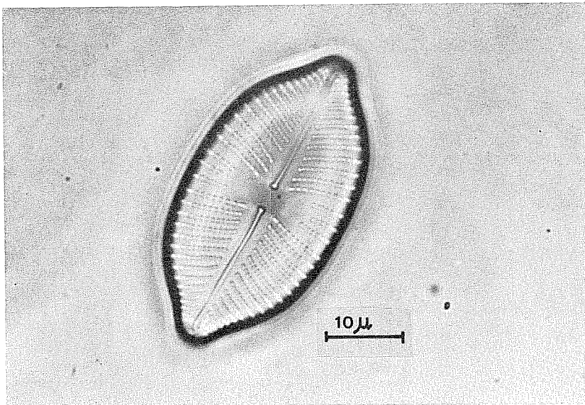
Fig. 2 - Navicula amphibola Cleve
