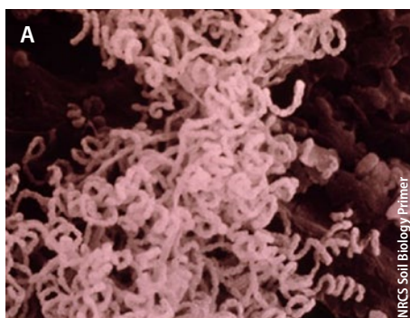
Examples of organisms that enhance soil health include (A) actinomycete bacteria, which decompose organic matter into compost (0.0005 mm), (B) turtle mites (Orobatiidae), which shred plant material into pieces, facilitating decomposition (0.05 mm), and (C) predatory nematodes (Monochidae), which regulate populations of pest nematodes (3 mm).
