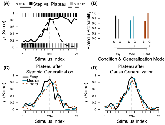
Figure 4: Identification Patterns by Generalization Model and Condition. See text for explanation.
