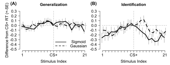
Figure 5: Response Times (RT) in Generalization and Identification. Y-axis represents RT(Stimulus) minus RT(CS+) calculated on the log-scale (positive = slower than for CS+). Error bars = +-1SE. Gray vertical line = CS+ location, gray horizontal = zero difference reference point.
