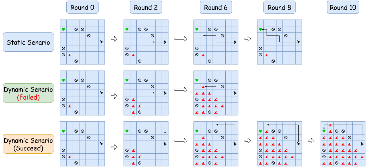
Figure 1: This is a case of scenarios involving dynamic elements that influence decision-making. In the figure, \times represents the starting point, \heartsuit represents the target point, and \odot represents walls or obstacles. Additionally, there is a spreading \blacktriangle , which expands by one grid every two rounds. In the presence of only static elements, the shortest path length is 8. However, when dynamic elements such as fire are introduced, the previously optimal path becomes unsafe. Therefore, it is essential for large language models to anticipate this situation and select an alternative route in advance, resulting in a new shortest path length of 10.
