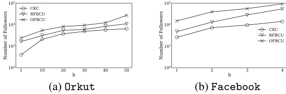
Figure 8: (Eval-III) Followers for varying b .
