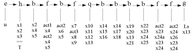
Figure 6: Communication protocol of Mathew at context c_1 .
