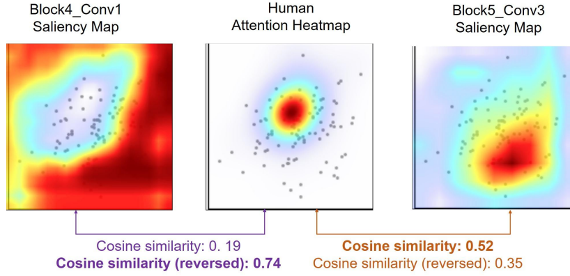
Figure 6: Human participants' attention heatmap and VGG-19 40K saliency maps in an example trial in He et al. (2025) datasets.
