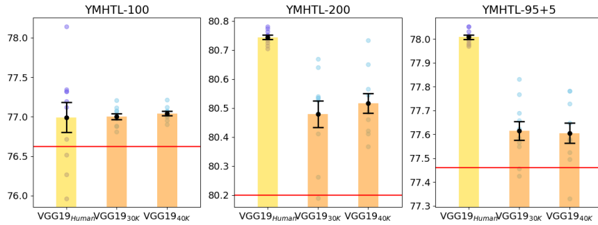
Figure 7: Models' predictive accuracy (%) of the three correlation discrimination datasets from Yang, Ma et al. (2023). The horizontal red lines represent the accuracy of the baseline model that always selected the scatterplot with the highest correlation. VGG19 Human represents Yang, Ma, et al.'s (2023) model trained on human data. Error bars denote standard errors.
