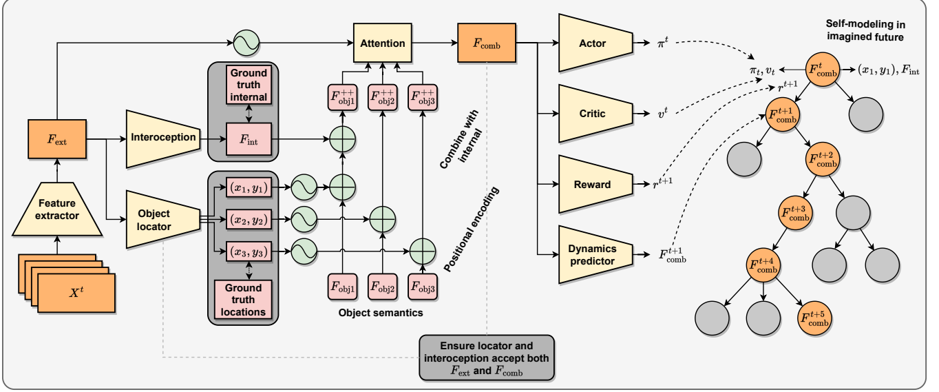
Figure 2: Architecture of SubjectZero. A convolutional feature extractor obtains high level features F_{ext} from the visual sensory inputs. An object locator predicts object coordinates from those features. They are trained in a supervised manner with the ground truth locations. The predicted object coordinates are encoded and added to a number of learned object representations F_{obj} . An interoceptive component produces features F_{int} which are supervised by the reward function, or a similar signal modeling the agent’s body. They are added to the object corresponding to the agent itself. Subsequently, an attention block aggregates all available features, producing F_{comb} . From it, an actor, critic, reward, and dynamics network branch out. Their outputs are used by the Monte Carlo Tree Search (MCTS), similar to MuZero. Yellow components are learnable networks. Red components are explicit and interpretable semantic objects meaningful in the world model. Orange objects are latent signals which are not interpretable but are useful for processing. Most time indices for the current step are omitted for clarity.
