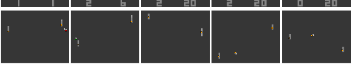
Figure 3: Predictions. We showcase samples from different test runs. The player is the right paddle. Scores are shown at the top. In all cases the agent accurately predicts the object visibilities and locations. The ball is colored green, red, or orange based on the agent’s own prediction of whether the current observed state is beneficial, harmful, or neutral, as given by the interoception module. Overall, the agent learns to play Pong effortlessly while at the same time being able to self-localize.
