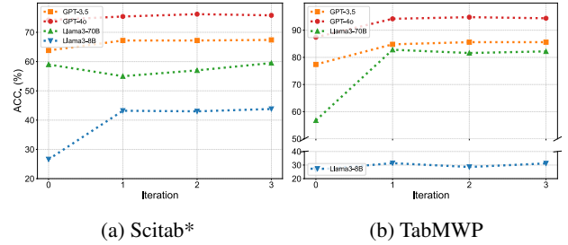
Figure 3: Iterations on 2 example datasets.
