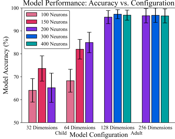
Figure 3: Model performance, in terms of accuracy, under each configuration (see also Table 1). Bars are the mean across all trials and ranges are the standard error of the mean.
