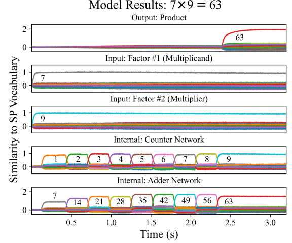
(a) Correct repeated addition (adult, n_n = 200 , n_d = 128 ).
