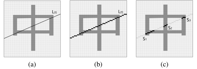
Figure 1: RLSWSA steps: (a) Line generation, (b) Pixel traversal, (c) Segment identification.
