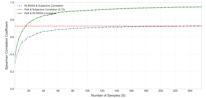
Figure 4: Correlation between RLSWSA and Traditional Algorithm Complexity Measurements at Different Sampling Counts.
