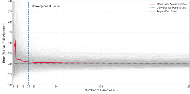
Figure 3: Percentage error distribution of RLSWSA compared to the Pelli algorithm for perimeteric complexity calculation at different sampling counts. Individual symbol error trajectories are shown by thin lines, and the average error by the thick red line. The convergence point is indicated at S=24 .
