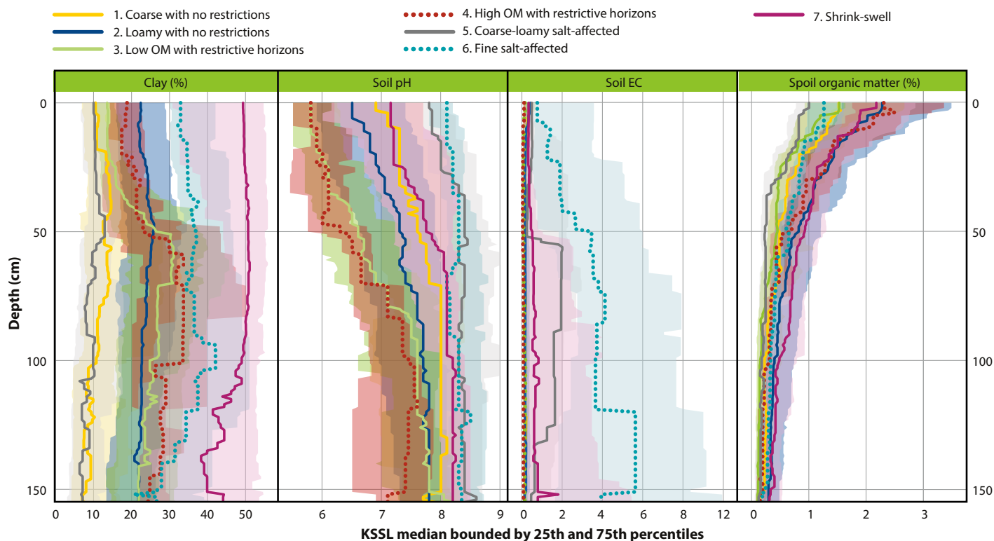
FIG. 2. Inherent soil properties differ by soil health region based on 369 validation locations from the Kellogg Soil Survey Laboratory (KSSL) database, emphasizing the need for a regional soil health approach. Most data was available in loamy with no restrictions ( n = 109 ), low organic matter (OM) with restrictive horizons ( n = 85 ), and shrink-swell ( n = 64 ) regions. Fewer points were available in coarse with no restrictions ( n = 41 ), fine salt-affected ( n = 28 ), coarse-loamy salt-affected ( n = 27 ), and high OM with restrictive horizons ( n = 15 ) regions. Soil organic matter (SOM) was estimated by multiplying soil organic carbon concentrations by the van Bemmelen factor (1.72). Solid lines are KSSL medians and shaded areas in the same color are 25th and 75th percentile values at 1-cm depth intervals.
