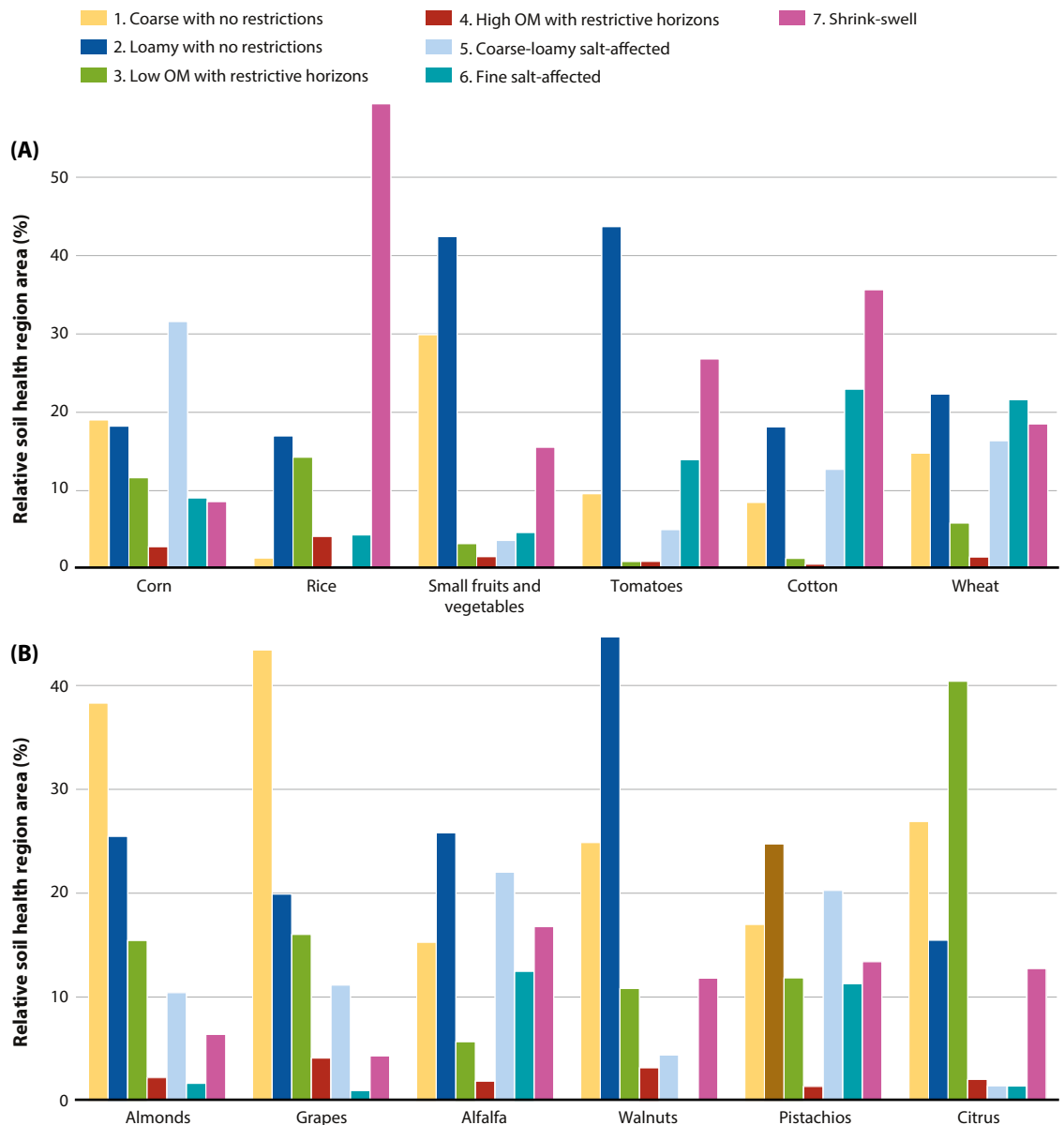
FIG. 5. Top six (by irrigated land area) annual (A) and perennial (B) crop types with proportions by seven soil health regions. Land use was identified by 2014 remote sensing (CDWR 2017), which classified 64% of the 5,274,720-ha study area.
