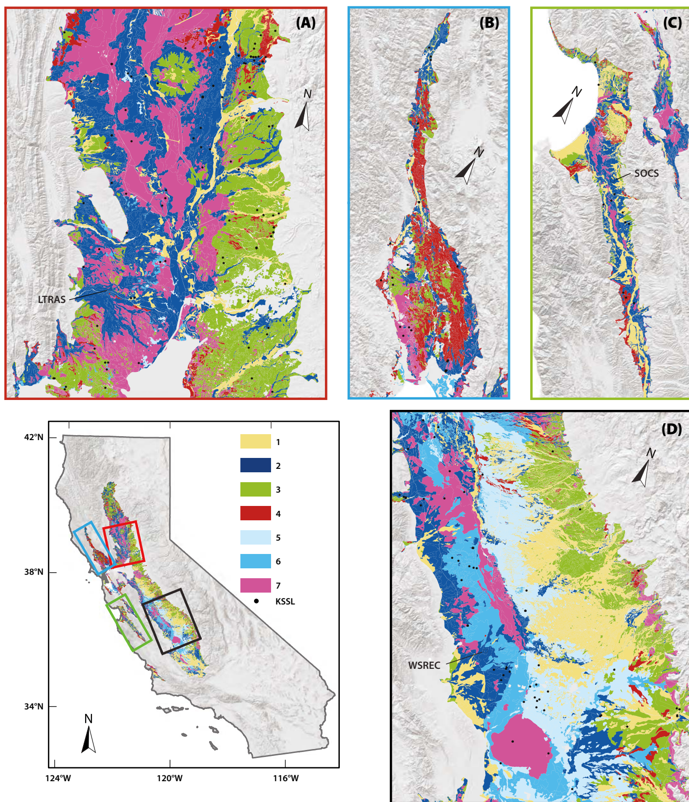
FIG. 1. Seven California soil health regions identified from cluster analysis of 10 soil properties derived from USDA-NRCS SSURGO (Soil Survey Geographic) data, highlighting the following: (A) southern Sacramento Valley, (B) Napa and Sonoma valleys (including adjacent hillsides), (C) Salinas, Santa Clara and Pajaro valleys and (D) central and southern San Joaquin Valley. Locations of Kellogg Soil Survey Laboratory (KSSL) points and three soil health experiments are depicted: the Long Term Research in Agricultural Sustainability (LTRAS), Salinas Organic Cropping Systems (SOCS) and UC West Side Research and Extension Center (WSREC). Soil health regions: 1 = Coarse with no restrictions, 2 = loamy with no restrictions, 3 = low organic matter (OM) with restrictive horizons, 4 = high OM with restrictive horizons, 5 = coarse-loamy salt-affected, 6 = fine salt-affected and 7 = shrink-swell.
