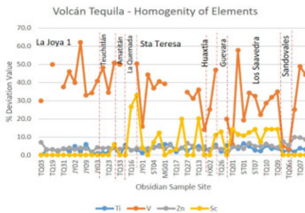
Figure 8. Variability in elements Ti, V, Zn, and Sc.
